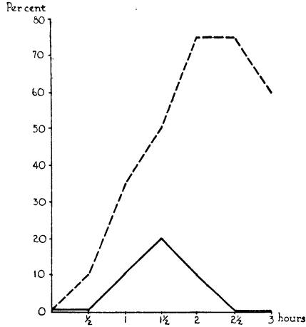
Chart I. Ordinate: percentage of B. prodigiosus appearing in caecum after intra-duodenal injection. Abscissa: time in half-hour intervals. Continuous line represents relative concentration of B. prodigiosus in ordinary temperature room. Broken line represents same in hot and humid room. Each graph is an average of nine experiments; three experiments were repeated using three different dogs.
