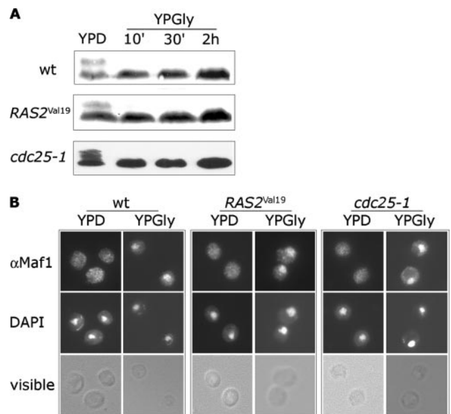
FIG. 4. Dephosphorylation and nuclear localization of Maf1 under respiratory conditions. (A) The wild-type strain YPH500 and the RAS2 Val19 and cdc25-1 mutants were grown to exponential phase in rich glucose medium (YPD), then transferred to prewarmed rich glycerol medium (YPGly), and further incubated at 30°C. Crude extracts from trichloroacetic acid-precipitated cells were analyzed by SDS-PAGE with a modified acrylamide-bisacrylamide ratio, followed by immunoblotting using polyclonal anti-Maf1 antibodies. The slower-migrating diffuse band corresponds to phosphorylated forms of Maf1. The phosphorylation pattern of Maf1 in the cdc25-1 mutant was identical to that observed for the isogenic A364A control strain (not shown). (B) Maf1 localization was analyzed by immunofluorescence microscopy using polyclonal anti-Maf1 antibodies. Cells were grown in glucose medium (YPD) to exponential phase, then transferred to glycerol medium (YPGly), and incubated for 2 h. Nuclei were stained with DAPI.
