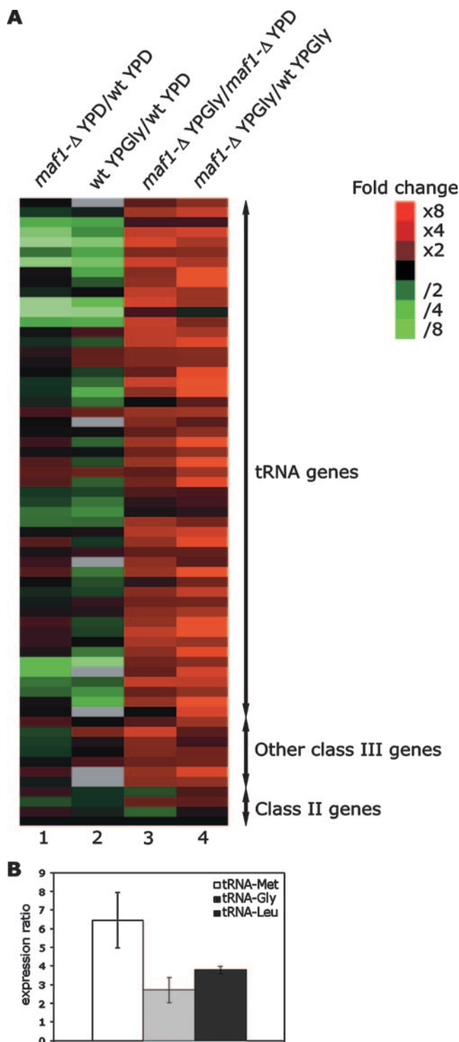
FIG. 3. Pol III genes are not equally regulated by Maf1. (A) Microarray hybridization. Expression ratios of Pol III-transcribed genes in the maf1-Δ mutant and the wild-type (wt) control strain (YPH500) grown in glucose medium (YPD) or glycerol medium (YPGly) with a shift to 37°C are shown. Results are presented according to the red-green color scale. Gray bar, not determined. (B) Comparison of expression of selected tDNA genes, tDNA Met (tM[CAU]J1), tDNA Gly (tG[UCC]G), and tDNA Leu (tL[CAA]A), in the maf1-Δ and the wild-type YPH500 cells, determined by real-time PCR. Expression levels were normalized to those of the control 35S rDNA. The relative expression ratios and standard deviations were calculated using the Relative Expression Software Tool.
