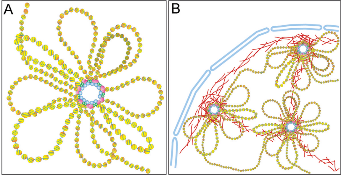
Figure 1. Insulator elements organize the chromatin fiber in the nucleus by establishing separate compartments of higher-order chromatin structure
