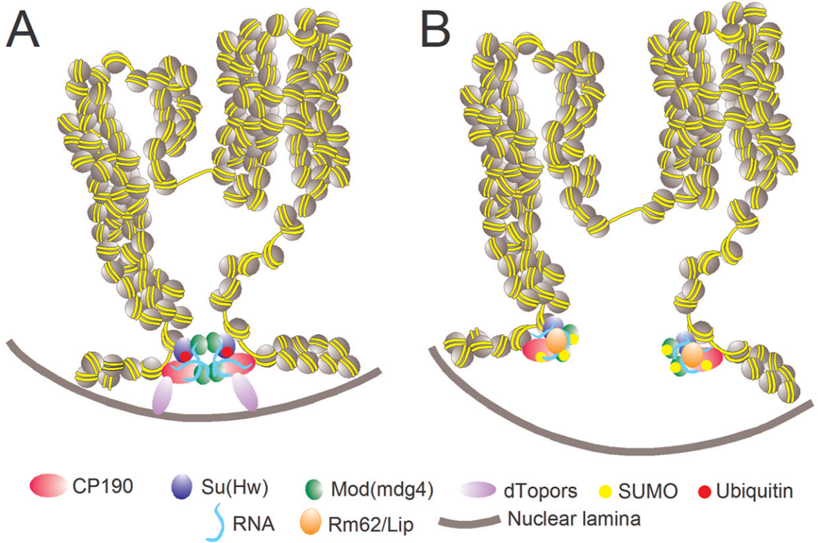
Figure 2. Insulator activity can be regulated by ubiquitination and sumoylation of insulator proteins
