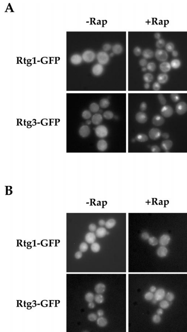
Figure 5. Rtg1 and Rtg3 are localized within the nucleus after rapamycin treatment in a TOR1 -dependent manner. (A) rtg1 \Delta (EY0733) or rtg3 \Delta (EY0735) cells expressing Rtg1-GFP or Rtg3-GFP, respectively, were treated with drug vehicle alone (left) or with 1 \mu g/ml of rapamycin (right) for 5 min, followed by examination by fluorescence microscopy. Pronounced nuclear accumulation of both Rtg1-GFP and Rtg3-GFP was observed in cells treated with rapamycin. (B) The experiment in A was repeated using cells that carried the dominant rapamycin resistant TOR1-1 allele.
