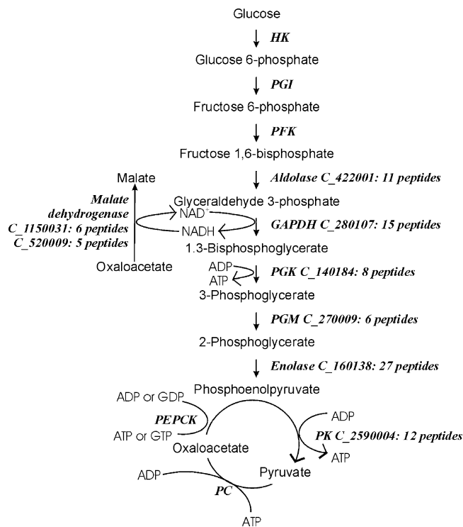
Figure 6. Enzymes of the glycolytic pathway found in the flagellar proteome. The number of peptides found for each protein is indicated. (HK) Hexokinase; (PGI) phosphoglucose isomerase; (PFK) phosphofructokinase; (GAPDH) glyceraldehyde 3-phosphate dehydrogenase; (PGK) phosphoglycerate kinase; (PGM) phosphoglycerate mutase; (PK) pyruvate kinase; (PC) pyruvate carboxylase; (PEPCK) phosphoenolpyruvate carboxykinase.
