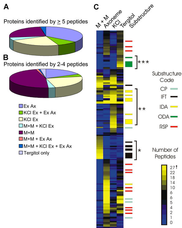
Figure 3. Distribution of proteins in flagellar fractions. (A and B) Distribution of proteins identified by five or more peptides (A) and by two to four peptides (B) in the extracted axoneme (Ex Ax), KCl extract (KCl Ex), and membrane + matrix (M+M) fractions. A protein was assigned to a specific fraction if it was identified by at least twice as many peptides in that fraction as in any other fraction. If the number of peptides in a second or third fraction was more than half that of the first fraction, the protein was assigned to two or all three fractions, as appropriate. Outer dynein arm subunits found exclusively in the Tergitol-insoluble fraction were automatically assigned to the KCl extract fraction. Seven additional proteins were identified by two to four peptides in the Tergitol-insoluble fraction only; these are included in B. (C) Hierarchical cluster diagram. Proteins were clustered based on the distribution of peptides in all four biochemical fractions. Each horizontal row represents one protein. The number of peptides in the particular fraction is represented by a color ranging from yellow (>27 peptides) to blue (0 peptides). In addition, the major known flagellar proteins are color coded under "substructure" with central pair (CP) proteins being marked in blue gray, intraflagellar transport (IFT) proteins in black, inner dynein arm (IDA) proteins in yellow, outer dynein arm (ODA) proteins in green and radial spoke proteins (RSP) in red. Note, for example, the IFT protein cluster (*) where nearly all peptides were found in the M+M fraction, the inner dynein arm cluster (**) where most peptides were most abundant in the KCl extract, and the outer dynein arm cluster (***) where nearly all peptides were found in the Tergitol-insoluble fraction. Only proteins represented by 15 or more peptides were included in the cluster analysis. A detailed version of this figure including gene IDs is available at http://labs.umassmed.edu/chlamyfp/index.php .
