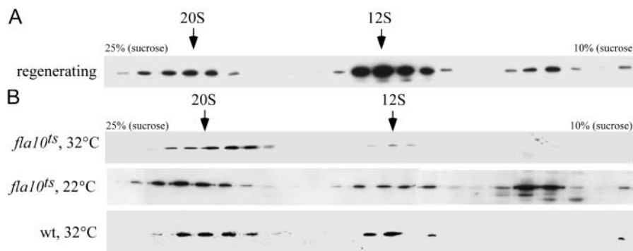
Figure 3. Radial spoke proteins enter the flagellum as a 12S complex.
