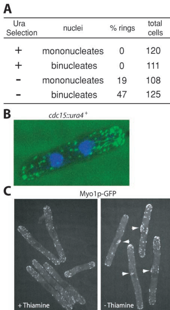
Figure 6. Cdc15p is required for formation of the medial actin ring. (A) Spores from the heterozygous cdc15 + /cdc15::ura4 + diploid were released into selective media (–uracil), indicated by +, or nonselective media (YE), indicated by –, and after 16 h were fixed and stained with AlexaFluor 488–phalloidin. The presence of a CAR in germinated cells was determined in binucleates and mononucleates. (B) A representative image of a binucleate cdc15::ura4 + cell, fixed and stained with AlexaFluor 488–phalloidin to visualize actin (green) and DAPI to visualize DNA (blue). (C) Myo1p–GFP localization in G2-arrested cdc25-22 cells either expressing (induced) or not expressing (uninduced) nmt1cdc15 .
