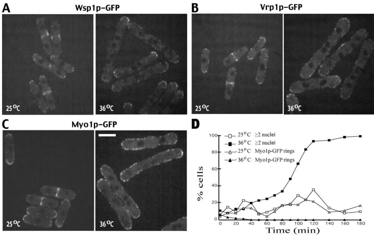
Figure 1. GFP-tagged Arp2/3 activators fail to localize to the medial region in a cdc15 mutant at the restrictive temperature. (A–C) cdc15-140 cells with either wsp1-GFP (KGY358), vrp1-GFP (KGY108), or myo1-GFP (KGY3963) alleles were grown to log phase at 25°C and shifted to 36°C for 4 h before live cells were imaged. Bar, 5 \mu m. (D) myo1-GFP cdc15-140 cells (KGY3963) were synchronized by lactose gradients and released to 25°C or 36°C. Live cells were monitored for Myo1p–GFP, and parallel samples were fixed and stained with DAPI. Localization of Myo1p to the medial region is indicated by triangles, and cells with two or more nuclei are indicated by squares.
