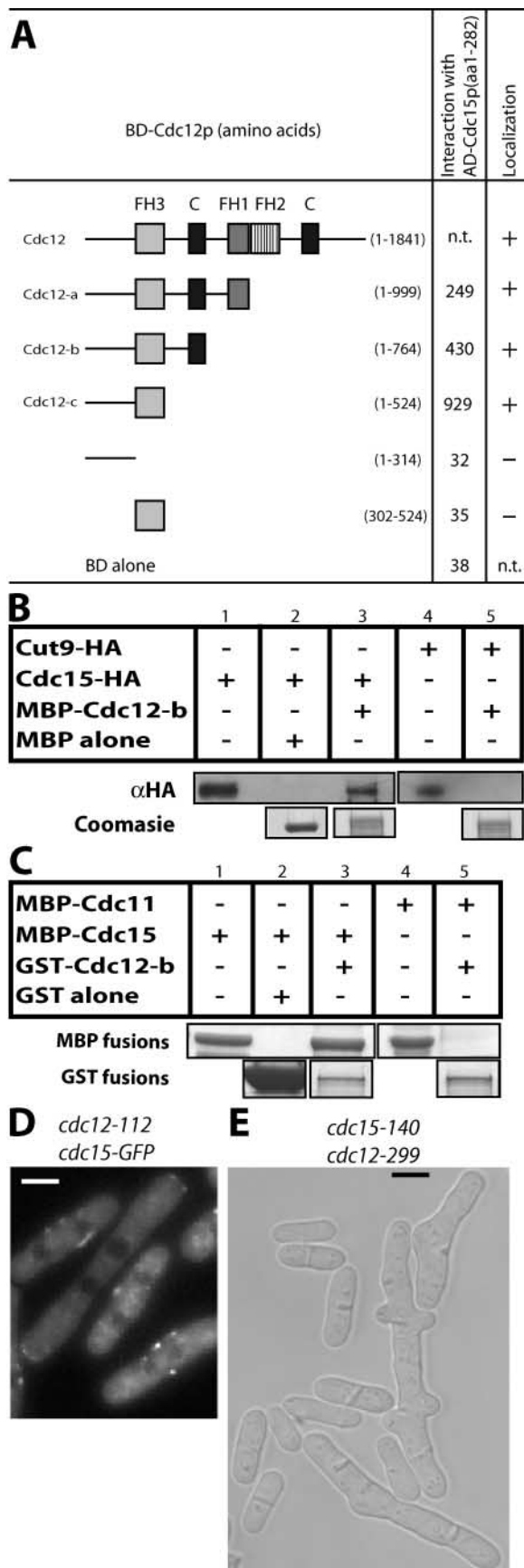
Figure 5. Cdc15p interacts directly with Cdc12p. (A) The indicated regions of Cdc12p were tested for interaction with Cdc15p (amino acids 1–282) by two-hybrid analysis. LEU + TRP + transformants were
