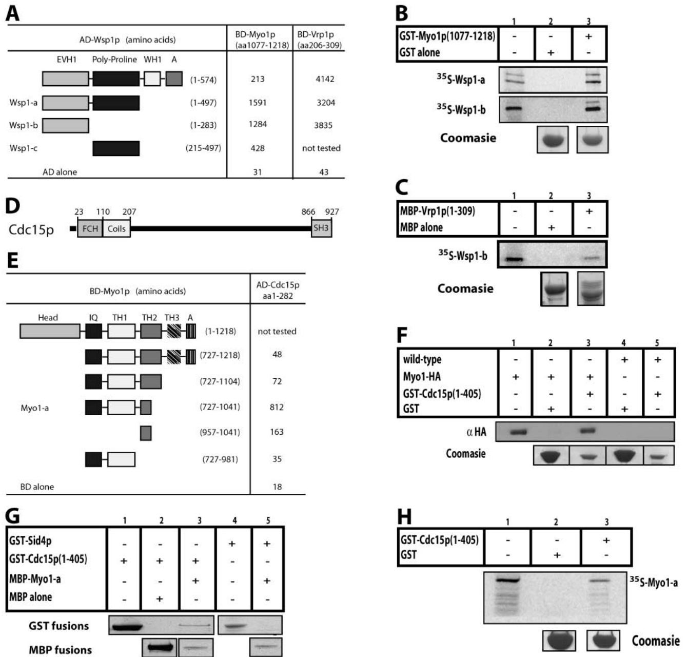
Figure 2. Protein-protein interactions of Arp2/3 complex regulators. (A) The indicated regions of Wsp1p were tested for interaction with Myo1p and Vrp1p by two-hybrid analysis. LEU + TRP + transformants were tested for growth on selective media (not depicted) and assayed for \beta -galactosidase activity measured in relative light units. (B) Approximately equal amounts of GST (lane 2, bottom) and GST-Myo1p(1077-1218) (lane 3, bottom) bound to glutathione beads were mixed with in vitro-translated Wsp1p-a (amino acids 1-497) (top) or Wsp1p-b (amino acids 1-283) (middle). Beads were collected, washed, and eluted as described in the Materials and methods. Proteins were resolved by SDS-PAGE and detected by fluorography (top two panels) or Coomassie staining (bottom). Only relevant portions of the Coomassie-stained gel are shown to indicate equal loading; however, all proteins ran at the predicted sizes. Lane 1 contains 10% of the input into the reactions. (C) Approximately equal amounts of MBP (lane 2, bottom) and MBP-Vrp1p(1-309) (lane 3, bottom) bound to amylose beads were mixed with in vitro-translated Wsp1p-b (top). Beads were collected, washed, and eluted as described in the Materials and methods. Proteins were further analyzed as in B. (D) A graphic representation of Cdc15p. Amino acid residues at the borders of known domains are shown. (E) The indicated regions of Myo1p were tested for interaction with Cdc15p (amino acids 1-282) by two-hybrid analysis. LEU + TRP + transformants were tested for growth on selective media (not depicted) and assayed for \beta -galactosidase activity. (F) GST (lanes 2 and 4) or GST-Cdc15p(1-405) (lanes 3 and 5) bound to glutathione beads were incubated with protein lysates from a myo1-HA strain (KGY3960) and subsequently extensively washed in binding buffer. Bound proteins were then divided and analyzed by immunoblotting (top) and Coomassie staining (bottom). Lane 1 contained lysate from myo1-HA strain and is an input control. (G) Approximately equal amounts of MBP (lane 2, bottom) and MBP-Myo1-a (amino acids 727-1041) (lanes 3 and 5, bottom) bound to amylose beads were mixed with either soluble GST-Cdc15p(1-405) (lanes 2 and 3) or GST-Sid4p (lane 5). Beads were collected, washed, and eluted as described in the Materials and methods. Proteins were resolved by SDS-PAGE and detected by Coomassie staining. Only relevant portions of the Coomassie gel are shown to indicate equal loading; however, all proteins ran at the predicted sizes. Lanes 1 and 4 contain samples of the GST fusion proteins before the binding reactions. (H) Approximately equal amounts of GST (lane 2, bottom) and GST-Cdc15p(1-405) (lane 3, bottom) bound to glutathione beads were mixed with in vitro-translated Myo1-a (top). Beads were collected, washed, and eluted as described in the Materials and methods. Proteins were further analyzed as in B.
