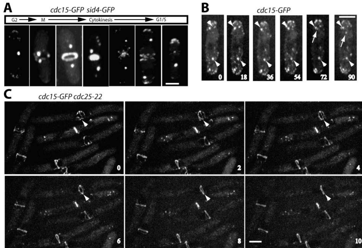
Figure 3. Localization of Cdc15p-GFP. (A) Representative live cell images of cdc15-GFP sid4-GFP cells (KGY3362) from various cell cycle stages. Sid4p-GFP localization was used to monitor spindle pole bodies and to indicate cell cycle stage of cells. (B) Time-lapse images of an interphase cdc15-GFP cell (KGY3019) with two nonmotile spots indicated by arrowheads. The arrow indicates the formation of a smaller patch from a larger one. Time is indicated in seconds. (C) Time-lapse images of synchronized cdc15-GFP cdc25-22 cells (KGY3042) that had been arrested for 4 h at 36°C and released to 25°C for 10 min before the beginning of the time course at the early stages of ring formation. The arrowhead indicates a branched network of fibers encircling the medial region that is the initial Cdc15p ring structure. This network then coalesced to form a thick bright ring structure. Time is indicated in minutes. Bars, 5 μm.
