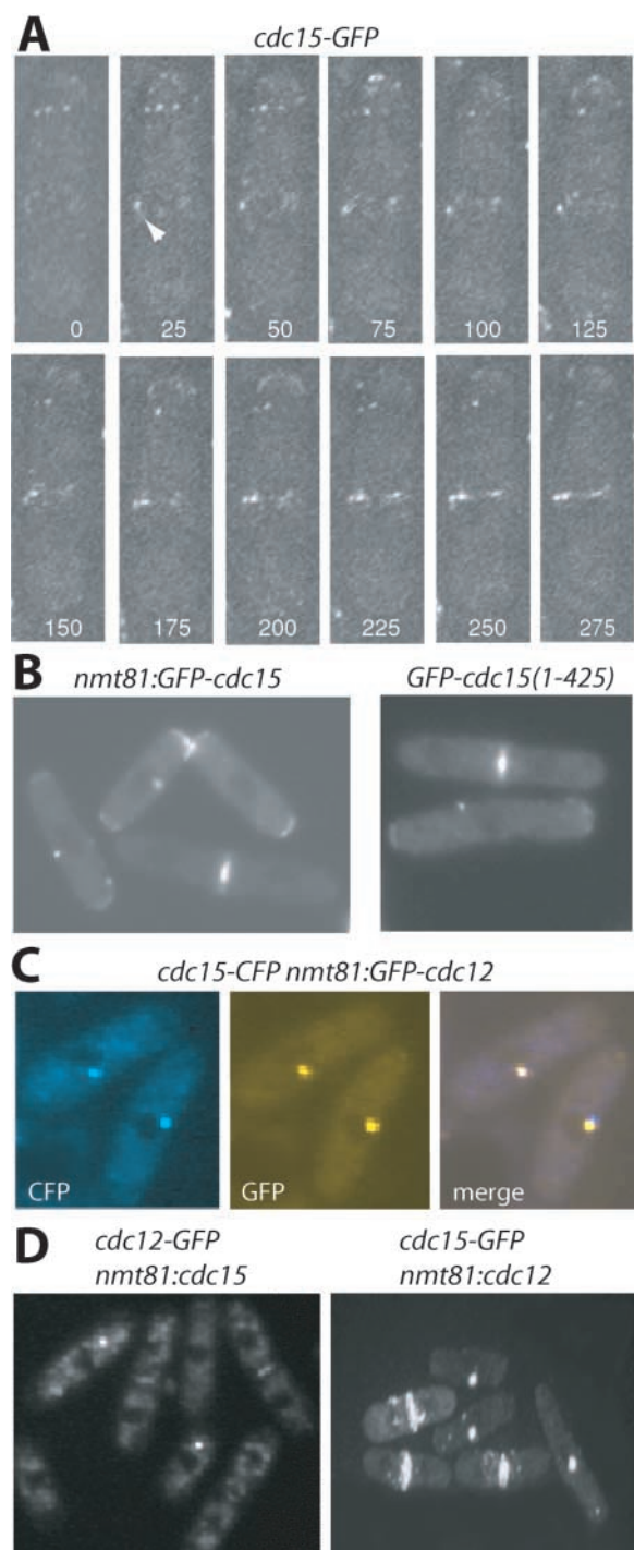
Figure 4. Cdc15p colocalizes with the formin Cdc12p in a medial spot. (A) Time-lapse images of a cdc15-GFP cell (KGY3019). The arrowhead indicates the initial localization of a Cdc15p–GFP spot to the medial region with subsequent incorporation of other Cdc15p patches into this structure. (B) GFP–Cdc15p, expressed under control of nmt81 promoter, and GFP–Cdc15p(1–425), under control of the cdc15 + promoter, were visualized in live wild-type cells. (C) GFP–Cdc12p was expressed under control of the nmt81 promoter and visualized in live cdc15-CFP cells (KGY3352). (D) Cdc15p was produced under control of the nmt81 promoter in cdc12p-GFP cells (KGY3066), and live cells were imaged (left). Cdc12p was produced under control of the nmt81 promoter in cdc15-GFP cells (KGY3019), and live cells were imaged (right).
