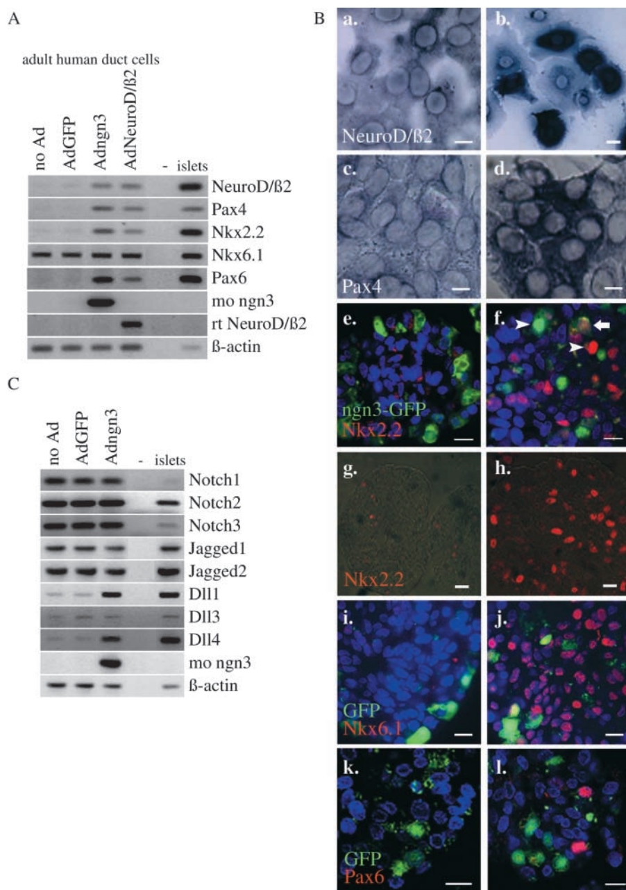
Figure 3. Effect of adenovirus-mediated ectopic expression of ngn3 or NeuroD/ \beta 2 on key transcription factors and signal transduction proteins in adult duct cells. (A) RT-PCR analysis of RNA encoding key developmental transcription factors from control and virus-infected duct cells and islets. Adngn3-expressed mouse ngn3 and AdNeuroD/ \beta 2-expressed rat NeuroD/ \beta 2. (B) Analysis of the effects of ngn3 (b, d, f, h, j, and l) compared with AdGFP-infected control cells (a, c, e, g, i, and k) at the cellular level by in situ hybridization of NeuroD/ \beta 2 (a and b) and Pax4 (c and d) mRNA and immunofluorescence for Nkx2.2 (e–h), ngn3 (e and f), Nkx6.1 (i and j) and Pax6 (k and l). Sections for immunocytochemistry underwent short (1 h) fixation to preserve GFP fluorescence. Arrowheads in panel f point to cells expressing either Nkx2.2 or ngn3 (intense red, respectively, green nuclear staining), and arrow points to a cell expressing Nkx2.2 and still containing GFP (weak green fluorescence in cytoplasm combined with weak red staining in the nucleus) without high level expression of ngn3 . Panels g and h represent a combination of phase-contrast and fluorescence microscopy (Nkx2.2 immunostaining), emphasizing the massive effect of ngn3 . Bars, 10 \mu m. (C) RT-PCR analysis of RNA encoding Notch, Jagged, and Delta isoforms from control and virus-infected duct cells and human islets.
