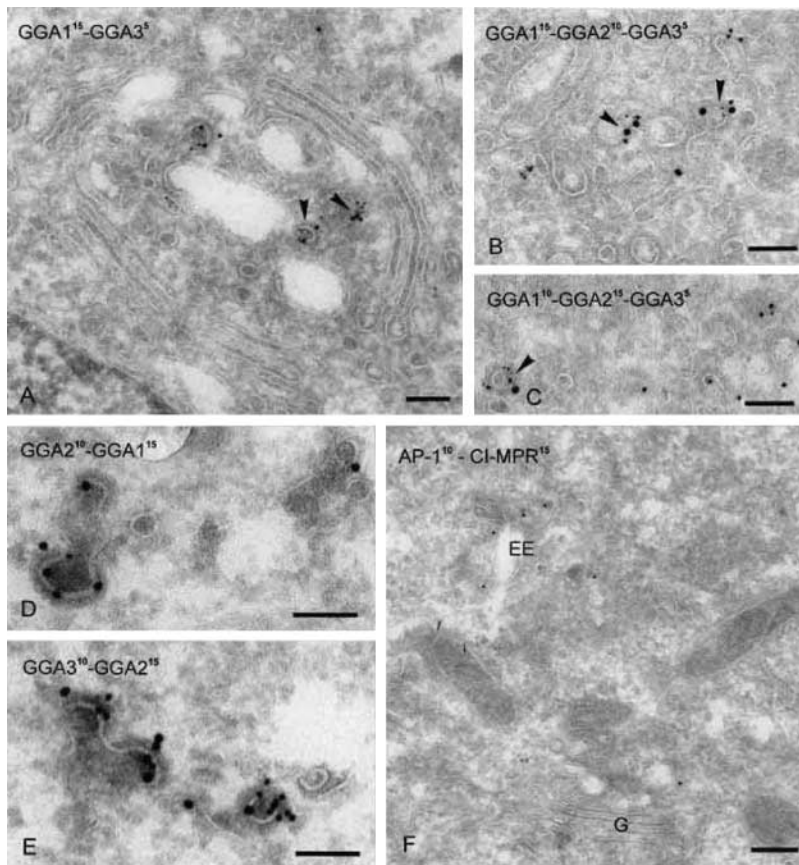
Figure 2. GGAs 1, 2 and 3 colocalize within the same coated buds at the TGN. Electron micrographs of immunogold-labeled cryosections showing the colocalization of GGAs (A–E) and the distribution of Cl-MPR and AP-1 in the trans-Golgi area of a GGA1 siRNA cell (F). (A–C) HeLa cells expressing myc-tagged GGA1. Using antibodies against myc, GGA2, and GGA3, double- and triple-labeling experiments with 5-, 10-, and 15-nm gold show that all three GGAs colocalize to coated pits and vesicles at the TGN (arrowheads). D and E show the colocalization of endogenous GGA1, 2, and 3 at coated buds on the TGN in HeLa cells. (F) AP-1 and Cl-MPR double immunolabeling in a GGA1-depleted HeLa cell. G, Golgi stack; EE, early endosome. Bars: (A–E) 100 nm, (F) 250 nm.
