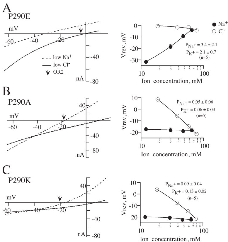
Figure 3. A negatively charged substitution at P290 (-2') results in cation-preferring receptors. (A) Amplitudes of GABA-induced currents from P290E were measured at a continuously varying membrane potential using the ramp protocol described in the Materials and methods. Ramps obtained in low sodium OR2 are the dashed lines and those in low-chloride OR2 are the solid lines. The normal OR2 ramp is omitted for clarity, but the reversal potential is indicated with an arrow. For the graph on the right, reversal potentials were measured at different concentrations of sodium (solid) or chloride (open) and fit with the GHK equation (Eq. 2) to determine the relative permeability coefficients. Substitution of negatively charged glutamate for the native proline at position 290 (-2') resulted in cation-preferring receptors, but receptors were chloride selective when this site was mutated to neutral alanine (B) or positively charged lysine (C).
