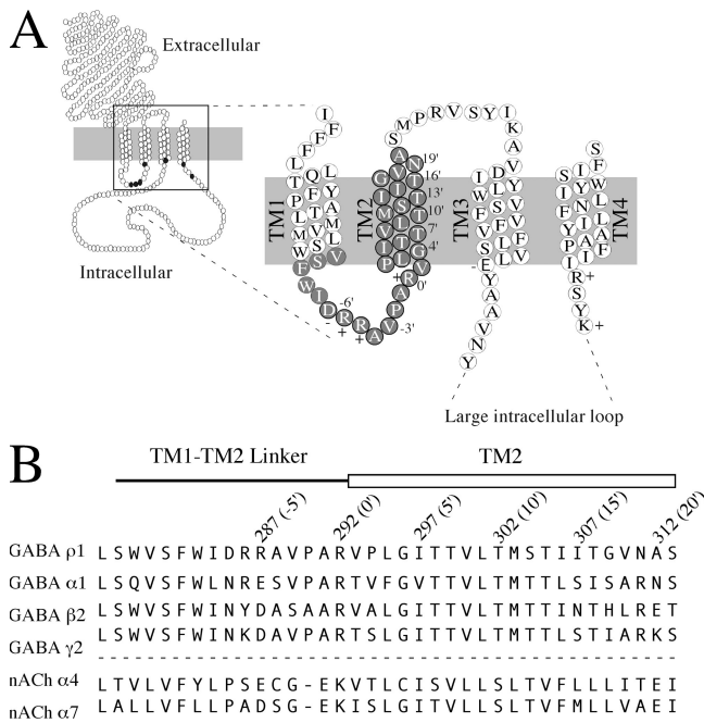
Figure 1. Diagram of proposed \rho 1 GABA receptor subunit topology and transmembrane domain sequences. (A) Endogenously charged residues are indicated by the appropriate charge sign and these residues were neutralized in this study to examine the role of endogenous charges on ionic selectivity. The TM2 numbering system used in the manuscript begins with the 0' TM2 arginine with increasing numbers proceeding toward the C terminus. Charge-scanning mutants covered the region from -12' (intracellular valine, V) to 20' (extracellular alanine, A) and are indicated with gray-filled circles. This figure is to merely show the extent of the residues examined in this study and the secondary structure or positions of these residues with respect to the membrane should not be taken literally. (B) Aligned TM1-TM2 linker and TM2 sequences from several representative members of the receptor family. Anionic members are above the dashed line, cationic members are below. The GABA \rho 1 receptor sequence is human, all others are rat.
