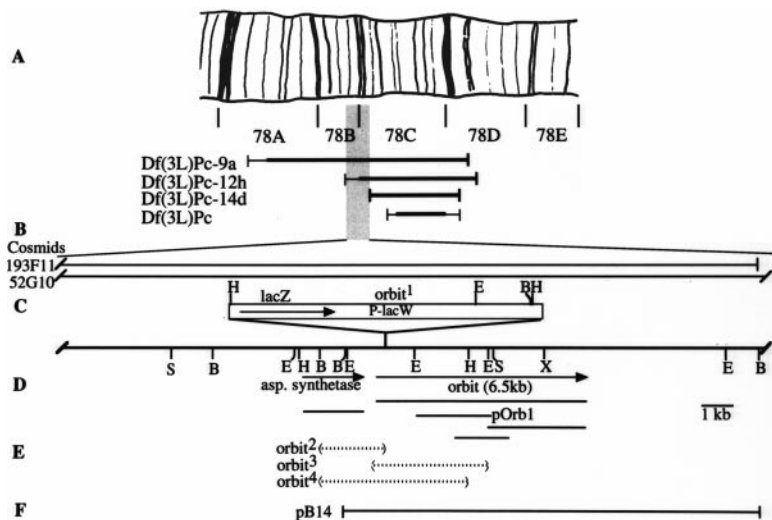
Figure 2. Cytological and physical maps of the orbit region. A, Polytene chromosome map of division 78. The cytological extents of the four deficiencies are shown as thick lines below the map. Thin lines indicate uncertainties in the deficiency breakpoints. The orbit mutation was uncovered by Df(3L)Pc-9a and Df(3L)Pc-12h , but not by Df(3L)Pc-14d or Df(3L)Pc . This places orbit within the chromosome interval 78B3-C1 to 78C2. B, Horizontal lines represent the genomic regions contained by two cosmid clones, 52G10 and 193F11. C, Restriction enzyme map of the orbit region. Cleavage sites are: B, BamHI; E, EcoRI; H, HindIII; S, SalI. D, Extents of the orbit and asparagine synthetase transcription units in which the arrowhead indicates the 3' end of the transcript. The cDNA clones for the two transcription units were isolated from 0–8- or 0–22-h embryonic cDNA libraries, or from a testis cDNA library. E, The extent of the genomic deletions associated with the three lethal alleles is represented as dotted lines between parentheses. The deletion associated with orbit 2 extends from within the 0.9-kb BamHI fragment in the aspartate synthetase gene to within the P element. The deletion associated with orbit 4 also extends from within the 0.9-kb BamHI fragment to a position within the 2.0-kb EcoRI–HindIII fragment of the orbit gene. The 3-kb deletion resulting in the orbit 3 mutation extends from the 5' regulatory region to within the 2.0-kb EcoRI–HindIII fragment of the orbit gene without affecting the function of the asparagine synthetase gene. F, The 14-kb BamHI fragment from cosmid 193F11 was used for germ-line transformation.
