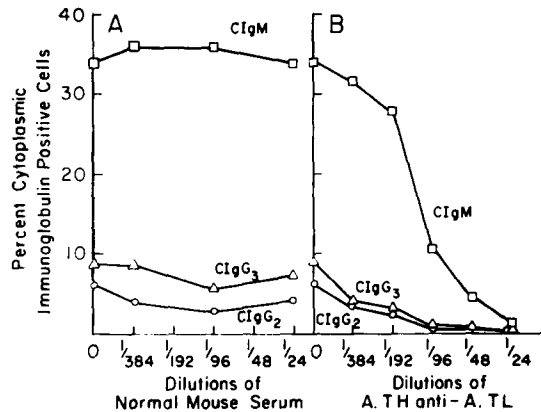
FIG. 2. Effects of normal CBA serum, (A) or A.TH anti-A.TL antiserum, (B) on the LPS induced differentiation of 1-day-old spleen cells to plasma cells synthesizing cytoplasmic IgM, —□—; IgG 2 , —○—; and IgG 3 , —△—. Anti-Ia serum and normal mouse serum were present at the indicated concentrations for the duration of culture.
