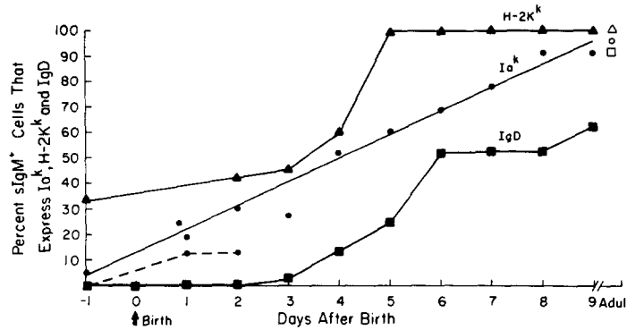
FIG. 1. Developmental relationships of H-2K k , Ia k , and IgD on splenic and liver B lymphocytes of fetal and neonatal CBA/J mice. Results are expressed as percentage of surface IgM + cells in spleen which stained with either anti-H-2K k , —▲—; anti-Ia k , —●—; or anti-IgD, —■—. Adult values are given on the right of the graph in open symbols. Fetal liver B lymphocytes stained with anti-Ia k are represented by the dashed line, --●--. IgM + B lymphocytes in liver were also examined for IgD but up until 2 days of age no surface IgD + cells were detected. When adult CBA/J spleen cells were incubated with normal mouse serum or anti-Ia k antiserum followed by RITC anti-γ1 or with RITC anti-γ1 alone, <0.5% of cells were stained.
