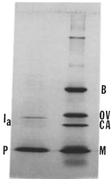
FIG. 4. SDS-PAGE of partially purified pili (12.5% gel). Gel purposely overloaded with 75 \mu\text{g} pili to detect contaminants. Stained with Coomassie Blue. Ia, protein Ia; P, pili. Molecular weight markers are BSA (B), ovalbumin (OV), carbonic anhydrase (CA), and sperm whale myoglobin (M).
