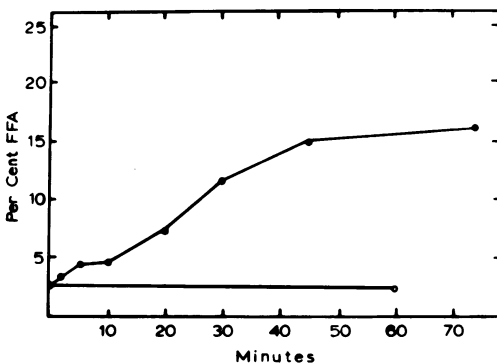
FIG. 3. Free fatty acid (FFA) formation after EDTA treatment of S15. The acyl groups of phospholipids were labeled by growth of the wild-type strain in media containing [ ^{14}\text{C} ]acetate. At various times after the treatment of the cells with EDTA, samples were removed for phospholipid extraction and fractionation as outlined in the text. Symbols: \circ , untreated; \bullet , EDTA treated.
