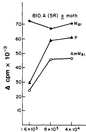
FIGURE 2. The response of B10.A(5R) anti-moth 81-103 PETLES to varying numbers of antigen-pulsed (pulsed) B10.A Percoll-enriched APC. Experimental details as in Table III. Antigens: moth 81-103 (M 81 , ●); pigeon 81-104 (P, ▲); acetimidyl moth 81-103 (AmM 81 , ○). Medium controls 1.6 × 10 3 APC/well: 6,300 ± 670; 8 × 10 3 APC/well: 18,500 ± 2,270; 4 × 10 4 APC/well: 26,900 ± 3,640.
