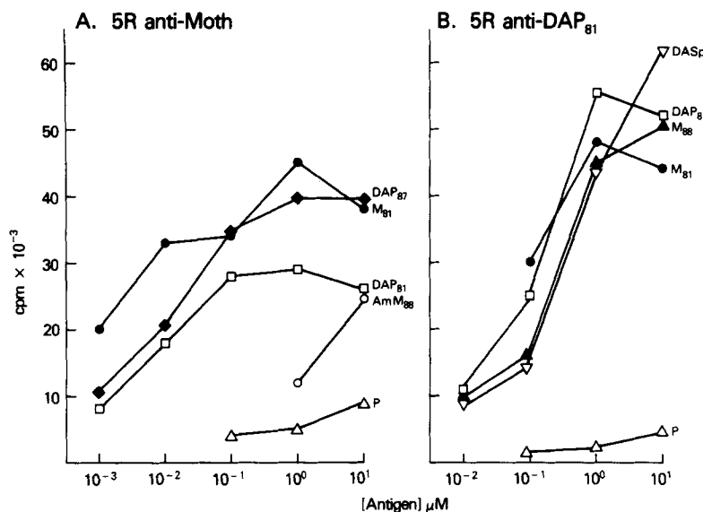
FIGURE 1. The specificity of the immune response of B10.A(5R) mice. B10.A(5R) mice were immunized with 50 \mu\text{g} of moth 81-103(A) or des-Ala 103 -pigeon (DAP 81 ) (B). After 9 d nylon wool passed lymph node cells were cultured with varying concentration of the antigen peptides for 72 h. During the last 12 h 1 \mu\text{Ci} of [ 3 H]thymidine was present. Antigens: des-Ala 103 -pigeon 81-104 (DAP 81 , \square ), moth 81-103 (M 81 , \bullet ), Am moth 88-103 (AmM 88 , \circ ), moth 88-103 (M 88 , \blacktriangle ), des-Ala 103 -splice (DASp, \nabla ), des-Ala 103 -pigeon 87-104, (DAP 87 , \blacklozenge ), pigeon 81-104 (P, \triangle ). Media controls: A, 8,300 \pm 3,500; B, 1,900 \pm 800; PPD stimulation: A, 67,700 \pm 5,800; B, 81,600 \pm 3,600 (cpm \pm SEM).
