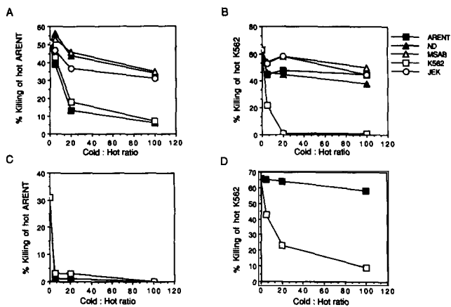
Figure 4. Effect of unlabeled (cold) target cells on the cytolytic activity of a CD3 - line and a CD3 - clone. Unlabeled target cells (K562, specific stimulator LCL ARENT, or irrelevant LCLs) were tested for their ability to inhibit the lysis of 51 Cr-labeled specific stimulator LCL ARENT (panel A for the line-D and panel C for the clone-3) or K562 cells (panel B for the line and panel D for the clone). An effector to 51 Cr-labeled target ratio of 12:1 for B, C, and D and 24:1 for A was maintained in all assays, as increasing numbers of cold inhibitor cells were added.
