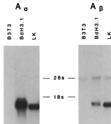
FIGURE 6. Comparable levels of Ia mRNA in LK-35.2 and BdH3.1 cells. Northern blots containing 4.0 \mu g RNA from BALB/c 3T3, BdH3.1, and LK-35.2 cells were hybridized to A_\alpha or A_\beta cDNA probes. Positions of 28 S and 18 S rRNA are shown.
