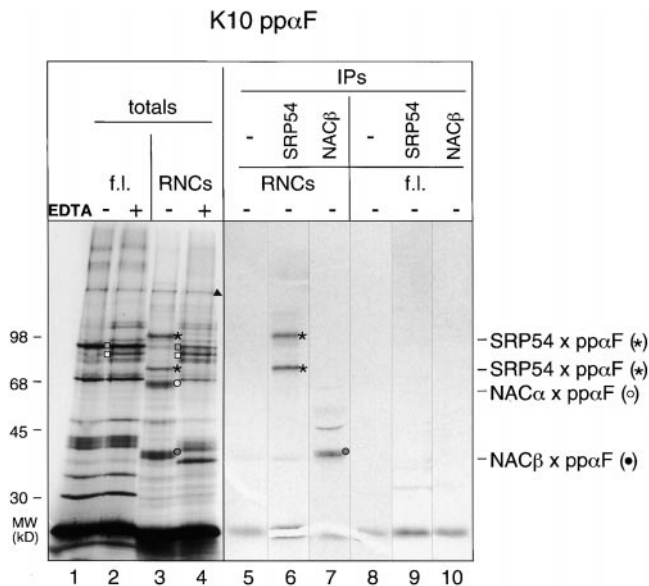
Figure 2. SRP and NAC only interact with RNCs. A fragment of 160 amino acids of pp \alpha F containing a single photoreactive lysine derivative at position 10 (K10 pp \alpha F) was synthesized in vitro. RNCs were isolated, and after addition of ribosome-depleted reticulocyte lysate were incubated with or without EDTA. Full-length (f.l.) pp \alpha F was synthesized in parallel and incubated with or without EDTA. After irradiation, the total products (totals) and products immunoprecipitated with antibodies to SRP54 or NAC \beta after denaturation in SDS (IP) were analyzed by SDS-PAGE. Control IPs were done without antibodies (-). The starting material for IPs was 3.5 that for the totals. Cross-linked products of pp \alpha F to SRP54 (*) and to the \alpha (○) and \beta subunits (●) of NAC are indicated. Cross-linked products of pp \alpha F to Hsp70 (■) and TCP1 \alpha (□) are also shown. The band marked with a triangle (▲) is an artefact of the gel.
