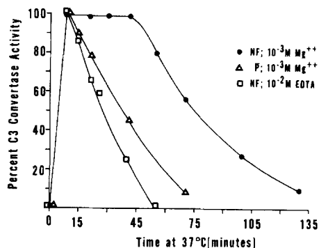
FIG. 3. Formation and decay of \bar{P} - and NF-C3 convertases as a function of time at 37°C. The Mg^{++} concentration was 10^{-3} M. In one experiment, EDTA was added to NF-C3 convertase 10 min after initiation of enzyme formation. At the indicated time intervals, 20 \mu l of the enzymes were sampled into 10 \mu l of EDTA solution containing 9.5 \mu g C3. C3 consumption was determined after 30 min at 37°C by effective molecule titration.
