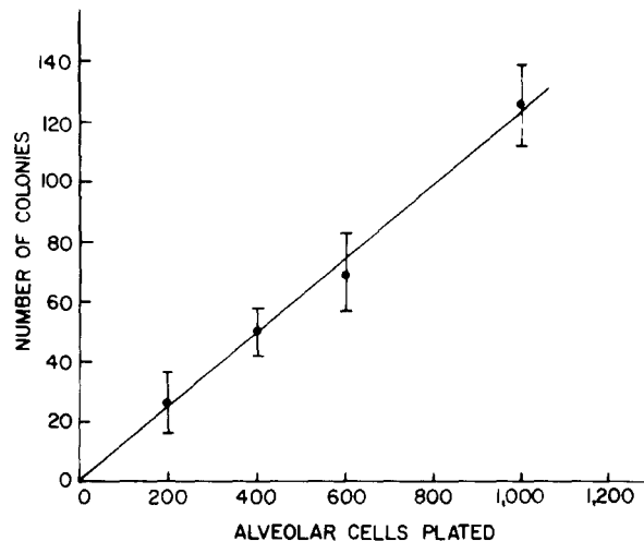
FIG. 2. Number of colonies formed as a function of alveolar cells plated. Error bars are 1 SD.
