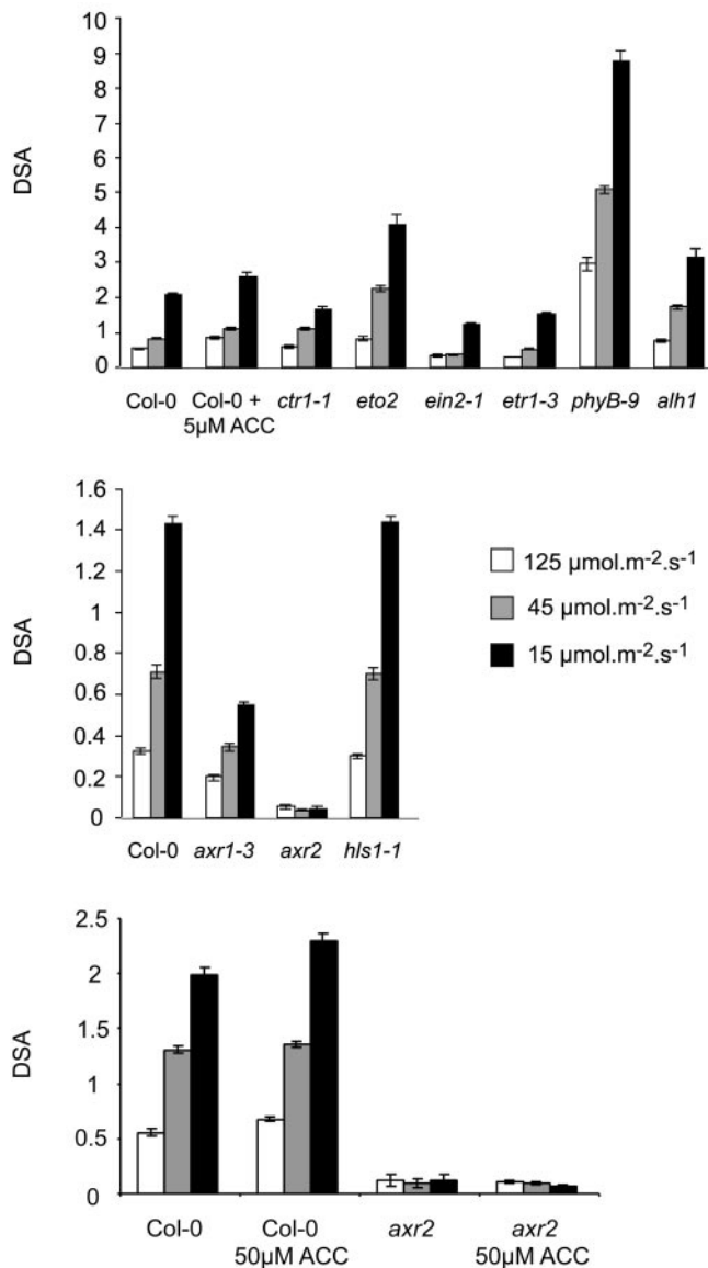
Figure 6. Comparison of biomass allocation in ethylene mutants (A), auxin mutants (B), and the effect of exogenous ACC (C), using a defined parameter: degree of similarity to shade avoidance (DSA). DSA = (\text{petiole length})^2 \times (\text{leaf blade surface area})^{-1} . Plants were grown for 1 week in 45 \mu\text{mol m}^{-2} \text{s}^{-1} PPF. After transfer (1.5 weeks) to 125 \mu\text{mol m}^{-2} \text{s}^{-1} (white bars), 45 \mu\text{mol m}^{-2} \text{s}^{-1} (gray bars), or 15 \mu\text{mol m}^{-2} \text{s}^{-1} (black bars), leaf 4 was analyzed for leaf blade surface and petiole length. Error bars = SE.
