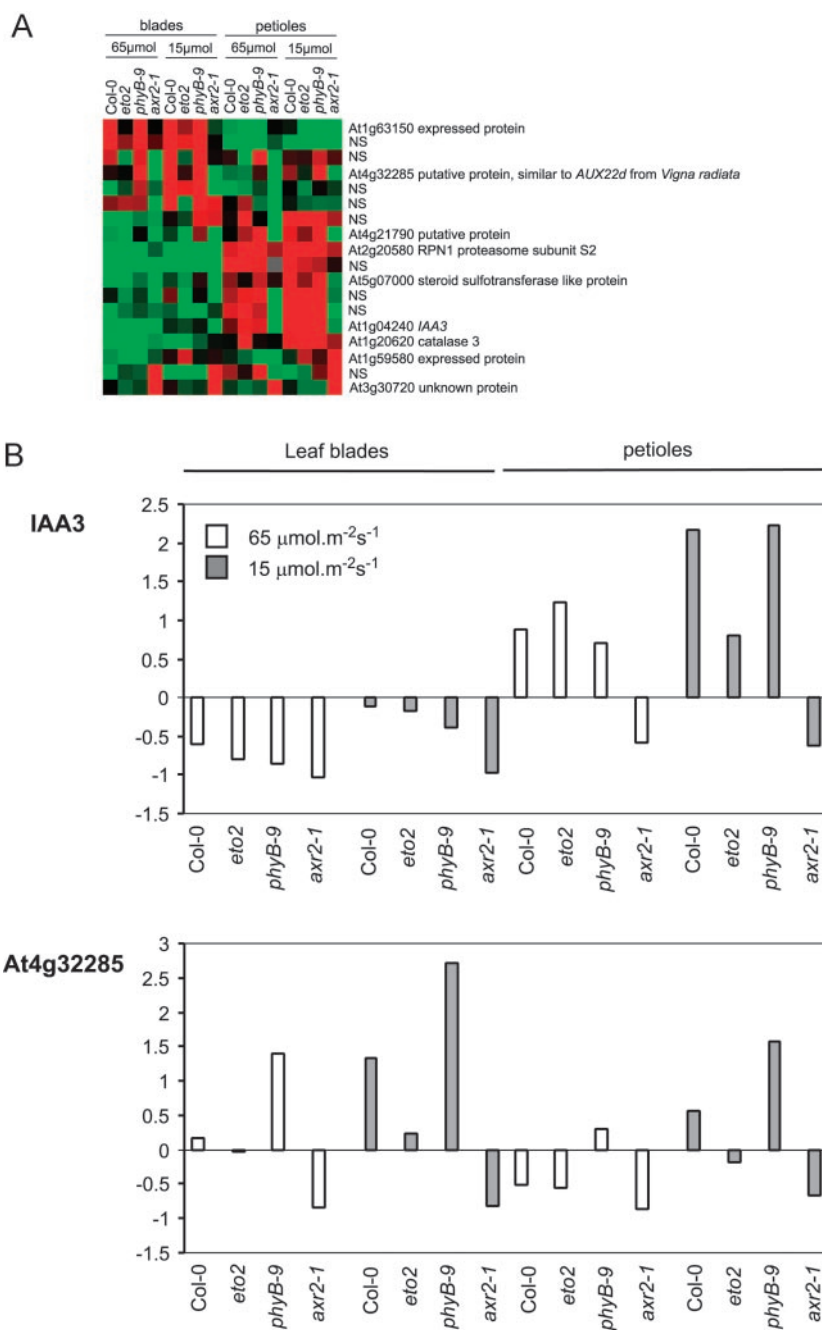
Figure 7. A, Cluster of shade-regulated fragments derived from cDNA-AFLP transcript profiling analysis. Colored squares, Relative transcript expression values of the genes in leaf blades and petioles of rosettes that were grown either in 65 or 15 \mu\text{mol m}^{-2} \text{s}^{-1} PPFD. Red, Up-regulated; green, down-regulated; black, neutral; gray, missing value. B, Histograms of the expression pattern in leaf blades and petioles of auxin-related genes IAA3 and At4g32285 derived from the semiquantitative analysis of cDNA-AFLP fragments, represented in A. Expression of the genes at a higher light intensity (65 \mu\text{mol m}^{-2} \text{s}^{-1} , white bars) and a lower light intensity (15 \mu\text{mol m}^{-2} \text{s}^{-1} , gray bars) are compared. Values are normalized and express the induction or repression compared with the mean of all samples, which is set as 0. The following formula was used: normalized value = (sample value - mean value of all samples) \times (sd of all samples) ^{-1} . A value lower than 0 represents a repression and higher than 0 an induction relative to the mean value of all tested samples.
