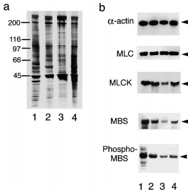
Figure 1. Gel electrophoresis and immunoblotting of stress fiber models with various antibodies. The whole cell extract (lane 1), Triton X-100-insoluble fraction of cells (lane 2), and model 1 (lane 3) and 2 (lane 4) stress fibers of human foreskin fibroblasts were electrophoresed and silver stained (a) or immunoblotted (b) with anti- \alpha -actin ( \alpha -actin), anti-MLC (MLC), anti-MLCK (MLCK), anti-MBS (MBS), or anti-phosphorylated MBS (phospho-MBS). Data indicate that all of these antigen polypeptides are associated with the cytoskeletal fraction and both stress fiber models. The amount of protein loaded to each lane was 2 \mu g for electrophoresis and 10 \mu g for immunoblotting.
