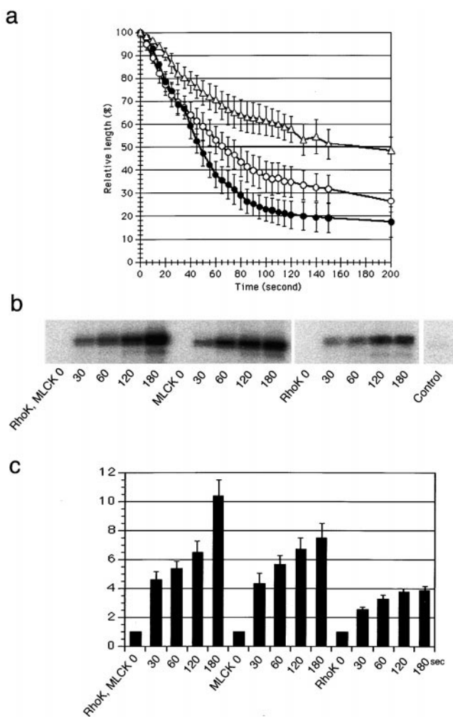
Figure 8. Rho-kinase and MLCK-dependent contraction of isolated stress fibers. (a) Stress fiber contraction by activating both Rho-kinase and MLCK (●), MLCK alone (○), or Rho-kinase alone (△). For details, refer to Results. The stress fiber length change expressed as a percentage of the original length was plotted against time. When both kinases were active, faster and more extensive contraction was observed. MLCK initiates contraction faster than does Rho-kinase. The values shown are means \pm SE of 10 individual isolated stress fibers. (b) Time courses of the MLC phosphorylation by both Rho-kinase and MLCK, MLCK alone, and Rho-kinase alone. Phosphorylation levels were determined by autoradiography at 0, 30, 60, 120, 180 s after the addition of radio-labeled ATP. Freshly isolated stress fibers were incubated for 180 s with Ca^{2+} -free Mg-ATP as a control. MLC phosphorylation was comparable to the level seen at time 0 of each experiment. 20 \mu\text{g} of protein was loaded in each lane. (c) Quantitative presentation of MLC phosphorylation under different conditions. The autoradiography bands were quantified by densitometry. The density of the band at time 0 was recorded as 1 for each series, and all the data are expressed relative to this value. The values shown are means \pm SE of four independent experiments.
