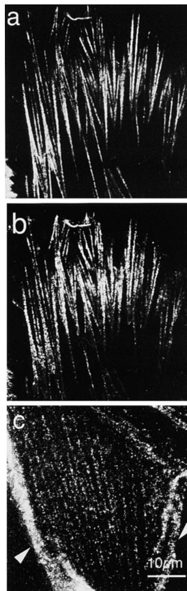
Figure 2. Immunofluorescence localization of myosin, MBS, and phosphorylated MBS in model 1 stress fibers. Stress fibers doubly stained with antimyosin (a) and anti-MBS (b) show dotted fluorescent patterns. When the two staining patterns were overlaid, many spots were superimposable. Banded anti-phosphorylated MBS staining is shown in c. Arrowheads in c indicate the peripheral stress fibers. Bar, 10 \mu m.
