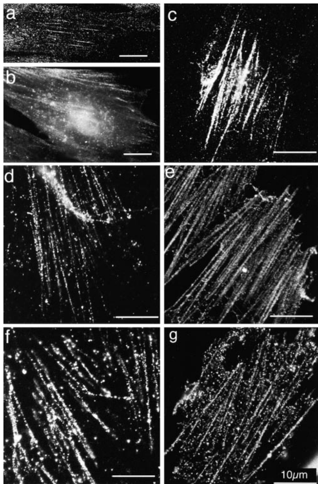
Figure 3. RhoA and Rho-kinase association with stress fibers. (a) A confocal image of stress fibers stained with anti-Rho-kinase (CC). The specimen was stained after the standard immunofluorescence procedure. (b) Cells were briefly extracted with Triton X-100 and stained with anti-Rho-kinase (CC). Using an epifluorescence microscope, stress fiber staining was detected against cytoplasmic staining. (c–e) Model 1 stress fibers treated with Triton X-100 for <3 min were stained with anti-RhoA (c) and anti-Rho-kinases, CC (d) and RB (e). Dotty staining along stress fibers was noted. (f and g) Model 2 stress fibers showed the similar dotted staining pattern with anti-RhoA (f) and anti-Rho-kinase (RB) (g). Bars, 10 \mu m.
