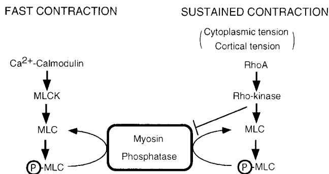
Figure 10. Two regulatory systems for actomyosin contraction in nonmuscle cells. P-MLC is phosphorylated MLC, which induces actomyosin-based contraction.
