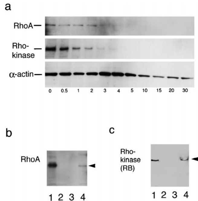
Figure 4. Extraction of RhoA and Rho-kinase from cells and stress fibers by Triton X-100. (a) Model 1 stress fibers were exposed to Triton X-100 for varying lengths of time (indicated in min) and analyzed for the content of RhoA and Rho-kinase by immunoblotting. RhoA and Rho-kinase were no longer detectable after 5 min of extraction. (b) RhoA, detectable in the whole cell extract (lane 1), could not be detected in the cell extracted by Triton X-100 for 10 min (lane 2). Although RhoA was not detected in model 1 stress fibers that were treated with Triton X-100 for 10 min (lane 3), it was associated with model 2 stress fibers (Lane 4). (c) Under these same experimental conditions, Rho-kinase was similarly extracted by Triton X-100. (a) Same amounts of TEA-treated samples were exposed to Triton X-100 for varying lengths of time. (b and c) 10 \mu g of proteins were loaded in each lane.
