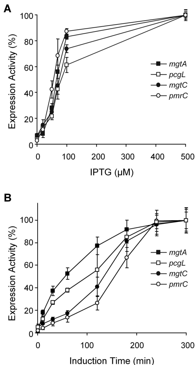
FIG. 4. PhoP- and \text{Mg}^{2+} -dependent expression of selected pag genes. Expression from the lacZ transcriptional fusions to mgtA , pcgL , mgtC , and the indirectly controlled gene pmrC was tested in a phoP::Tn10 background expressing PhoP from pEG9014 with addition of different concentrations of IPTG to the growth medium as indicated (A) and in a wild-type background (B), with aliquots withdrawn at different times as indicated, after transfer of the cells from a repressing (N-medium–12 mM \text{MgCl}_2 ) to an inducing (N-medium–8 \mu\text{M} \text{MgCl}_2 ) growth medium. \beta -Galactosidase activity from the corresponding lacZ transcriptional fusion was measured as described in Materials and Methods. Results are expressed as a percentage of the maximal expression achieved for each lacZ fusion and are averages from three independent assays performed in duplicate. Error bars, standard deviations.
