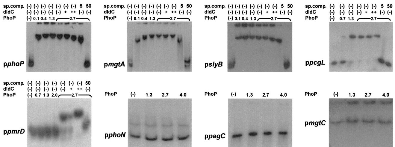
FIG. 3. PhoP binds to the promoter regions of the phoP , mgtA , slyB , pcgL , and pmrC genes but not to the promoter region of phoN , pagC , or mgtC . EMSA was performed using the ^{32}\text{P} 3'-end-labeled PCR fragment of the promoter region of phoP , mgtA , slyB , pcgL , pmrC , phoN , pagC , or mgtC , respectively, incubated with different amounts of purified PhoP-H6, in the absence or presence of different amounts of either poly(dI-dC) as a nonspecific competitor (didC) or the corresponding unlabeled PCR fragment (sp.comp.).
