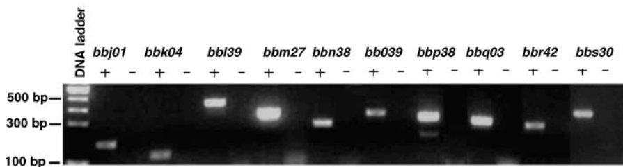
Figure 1. Amplification of selected B. burgdorferi lipoprotein genes that are expressed on the plasmids. Total RNA was prepared from cultured B. burgdorferi and analyzed by both PCR (-) and RT-PCR (+). PCR products were separated by ethidium bromide-incorporated agarose gel, and the lack of a product in the (-) column demonstrated that DNA was not present in the RNA preparation.
