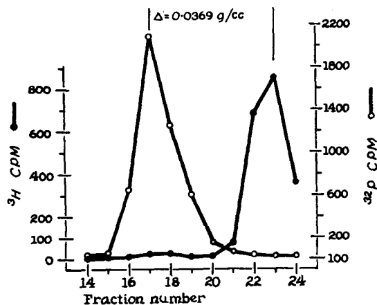
FIGURE 2. Distribution of radioactivity of heavy (open circles) and light (solid circles) DNA following CsCl density gradient centrifugation. The heavy DNA was labeled with ^{32}\text{P} and the light DNA with ^3\text{H} . Centrifugation, 60 hr at 32,000 RPM in an SW39 Spinco rotor.
