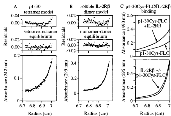
Figure 3. Sedimentation–diffusion equilibrium of p1–30 and soluble IL-2R \beta . Profiles of absorbance versus radius from the center of rotation were obtained by sedimentation–diffusion equilibrium at 25 krpm in 20 mM sodium phosphate, pH 7.2, at 20°C. Residual errors as a function of radial distance from the center of rotation show the fitting quality of the data to the selected models. (A) p1–30 initial concentration was 150 \mu M. Absorbance was recorded at 242 nm. A better fit was obtained with a tetramer–octamer model of equilibrium (bottom) than with a tetramer model (top). (B) IL-2R \beta 31–230 initial concentration was 14 \mu M. Absorbance was recorded at 295 nm. An equilibrium monomer–dimer model (bottom) seemed slightly better than a dimer model (top). (C) p1–30Cys-FLC and IL-2R \beta 31–230 initial concentrations were 150 and 14 \mu M, respectively. Absorbance of p1–30Cys-FLC (at 490 nm) in the presence or absence of IL-2R \beta 31–230 is shown (top). Profile at 295 nm (aromatic residue absorbance of IL-2R \beta 31–230) of the peptide–protein mixture is also shown (bottom).
