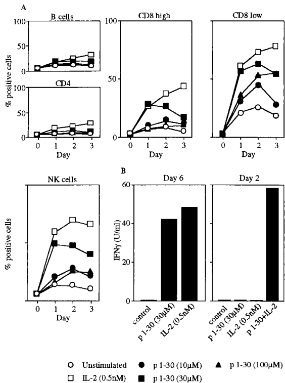
Figure 7. Activation of NK and CD8 T cells by p1-30 and induction of IFN- \gamma . (A) PBMCs were stimulated with IL-2 (0.5 nM) or p1-30 (10, 30, or 100 \mu M) for 1, 2, or 3 d. Subpopulations labeled with anti-CD4 (Th lymphocytes), CD8 (CTLs), CD20 (B lymphocytes), or CD56 (NK cells) were assayed for CD69 expression. Graphs represent the percentage of CD69 + cells for each population with respect to stimulant (IL-2 or p1-30) and time (day) of stimulation. Data of a representative experiment are shown. (B) IFN- \gamma production was measured on supernatants from PBMCs stimulated with IL-2 (0.5 nM) or p1-30 (30 \mu M) at day 6. In a second panel, synergy between IL-2 (0.5 nM) and p1-30 (30 \mu M) is shown after 2 d of stimulation.
