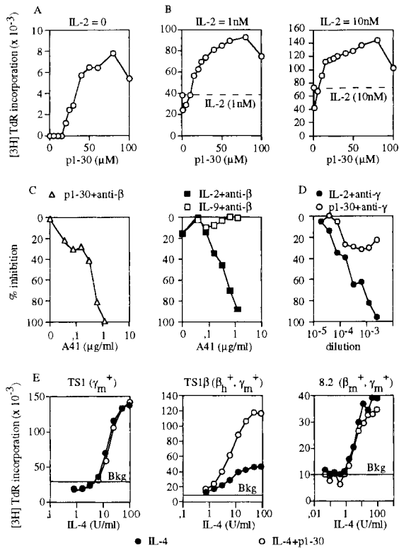
Figure 1. p1-30 induces cell proliferation and acts in synergy with IL-2. Role of human IL-2 \beta . TS1 \beta cells were stimulated with p1-30 (up to 100 \mu M) in the absence (A) or presence (B) of 1 or 10 nM IL-2. This was followed by measuring [ ^3 H]TdR incorporation. Proliferative responses induced with 1 or 10 nM of IL-2 were 38,148 and 72,370 cpm, respectively. Optimal responses were obtained with 60 \mu M of p1-30. Background was subtracted. (C) Effects of neutralizing anti-human IL-2R \beta mAb (A41) were tested on TS1 \beta cell proliferation induced by p1-30 (60 \mu M), IL-2 (1 nM), or IL-9 (10 nM). (D) Effects of two neutralizing anti-mouse IL-2R \gamma mAbs (3E12 and 4G3 mAbs) on the IL-2- and p1-30-induced proliferation of TS1 \beta cells. Abs isolated from mouse ascitic fluids were diluted and added to the cell culture. (E) Synergy between p1-30 and IL-4. Proliferative responses of TS1 (expressing mouse IL-2R \gamma ), TS1 \beta (expressing human IL-2R \beta and mouse IL-2R \gamma ), and 8.2 cells (expressing mouse IL-2R \beta and mouse IL-2R \gamma ) were induced at various concentrations of IL-4 (up to 100 U/ml) in the presence or absence of 60 \mu M of p1-30. Values obtained for p1-30 responses (Bkg) were subtracted from the IL-4 plus p1-30 response.
