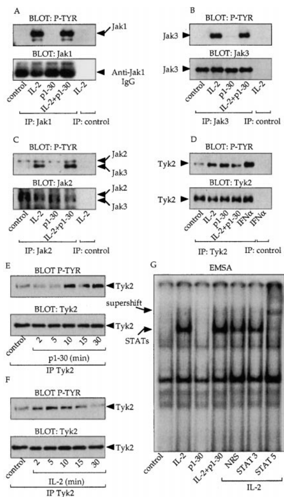
Figure 5. Implications of the Jak proteins in p1-30 signaling. (A–D) Analysis of Jak protein activation. Cells were stimulated for 10 min as indicated and immunoprecipitated with anti-Jak1 (A), Jak3 (B), Jak2 (C), and Tyk2 (D) mAbs. Antiphosphotyrosine blotting (P-TYR, top) and anti-Jak blotting (bottom) are shown. For C, the immunoblot displays two bands because the commercial anti-Jak2 serum cross-reacts with Jak3. However, the two kinases could be distinguished by their molecular weights. For D, cells were stimulated with IFN- \alpha (0.3 nM) as a positive control for Tyk2 activation. (E and F) Analysis of Tyk2. Kit 225 cells were stimulated for 2, 5, 10, 15, and 30 min with p1-30 (60 \mu M) or IL-2 (10 nM). After lysis and anti-Tyk2 immunoprecipitation, phosphotyrosine-containing Tyk2 was detected (top). The total amount of immunoprecipitated Tyk2 corresponding to each stimulation was verified (bottom). (G) Activation of STAT proteins by IL-2 but not by p1-30. EMSA was carried out on nuclear extracts of Kit 225 stimulated for 10 min with IL-2 (10 nM), p1-30 (60 \mu M), or both. Nuclear extracts were incubated with the GAS probe. Supershifted complexes were analyzed with antibodies directed against STAT5, STAT3, or a nonrelevant serum (NRS) after IL-2 stimulation.
