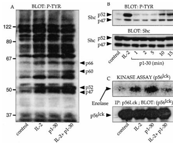
Figure 4. Signal transduction induced by p1-30. (A) General pattern of protein tyrosine phosphorylation. Kit 225 cells were stimulated for 10 min with IL-2 (10 nM), p1-30 (60 \mu\text{M} ), or both. Cells were lysed, and the pattern of protein tyrosine phosphorylation was visualized by SDS-PAGE and immunoblotted with mAb 4G10, specific for phosphotyrosine (P-TYR). Arrowheads indicate the phosphorylated proteins upregulated by p1-30. (B) Phosphorylation of Shc. Kit 225 cells were stimulated for 1, 2, 5, 10, and 15 min. After lysis, phosphotyrosine-containing proteins were detected with 4G10 mAb (top). The identity and equal loading of the two Shc isoforms were confirmed by probing with the mAb to human Shc (bottom). (C) Induction of p56 lck kinase activity. Kit 225 cells were stimulated for 15 min with 10 nM of IL-2, 60 \mu\text{M} of p1-30, or a combination of both. p56 lck was immunoprecipitated and tested for its ability to phosphorylate the exogenous enolase substrate (top). The bottom panel shows that equal amounts of immunoprecipitated p56 lck were used in the kinase assay.
