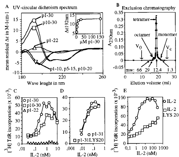
Figure 2. Structure–function analysis of p1–30. (A) The CD spectra from 180 to 260 nm are shown for p1–10, p5–15, p10–20, p1–22, p10–30, and p1–30 at 150 \mu M. The p1–30 concentration dependence (3–150 \mu M) of the CD signal at 192 nm is shown in the insert. (B) Size exclusion chromatography. Peptide p1–30 was eluted as a single main peak of molecular mass 13 kD (according to column calibration). Arrows indicate molecular weight (mw) markers, void volume ( V_0 ) and total volume ( V_c ). Monomeric, tetrameric, and octameric forms are shown. (C) TS1 \beta cell proliferation was tested at various concentrations of IL-2 (from 5 \times 10^{-3} to 10 nM) with 60 \mu M of either p1–30, p1–22, or p10–30. The response to IL-2 or peptide alone was subtracted from that obtained with both IL-2 and peptide. (D) Role of Asp20 in p1–31 activity. TS1 \beta cells were stimulated with various concentrations of IL-2 (from 5 \times 10^{-3} to 10 nM) in the presence of 60 \mu M of peptide p1–31 or p1–31(Lys20). Results are presented as in C. (E) The biological activity of mutant IL-2(Lys20) is shown for comparison.
