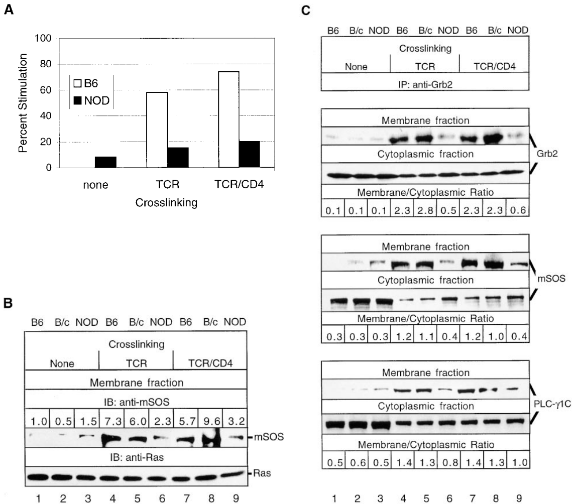
Figure 1. NOD thymocytes exhibit a constitutive reduction in mSOS activity due to its inability to be translocated from the cytoplasm to the plasma membrane. (A) mSOS was immunoprecipitated from the membrane fractions of NOD and B6 thymocytes ( 10^8 cells/lane) previously stimulated for 1.5 min by anti-TCR- \beta or anti-TCR- \beta plus anti-CD4. Ras GDP releasing activity associated with these immunoprecipitates was analyzed in vitro by determining the amount of released [ ^3 H]5'-GDP-Ras radioactivity in a nitrocellulose filter binding assay. Results are expressed as the percentage of change in mSOS GDP releasing activity relative to the basal level achieved in control samples ( none ). (B) NOD and control (C57BL/6J [B6] and BALB/c [B/c]) thymocytes were either not stimulated ( None ) or were stimulated for 1.5 min by anti-TCR- \beta or anti-TCR- \beta plus anti-CD4. Immunoblotting (IB) of thymocyte membrane fractions was performed with anti-mSOS and anti-Ras mAbs. Data are expressed as the relative fold change for the relative signal intensities calculated as a/b , where a is the specific signal intensity (density \times area/lane) obtained after TCR- \beta or TCR- \beta -CD4 cross-linking and b is the basal signal intensity (B6 control without cross-linking). (C) Membrane translocation of Grb2-bound mSOS and PLC- \gamma 1C is reduced in stimulated NOD thymocytes. NOD and control thymocytes were either not stimulated ( None ) or were stimulated as in B. Immunoblotting of Grb2 immunoprecipitates (IP) from thymocyte membrane and cytoplasmic fractions was performed with anti-Grb2, anti-mSOS, and anti-PLC- \gamma 1C mAbs. Data are expressed as the membrane/cytoplasmic ratio, calculated as a/b , where a is the relative signal intensity (density \times area) obtained for corresponding proteins precipitated from the membrane fraction, and b is the same value obtained after precipitation of proteins from the cytoplasmic fraction. The results shown are representative of one of two separate reproducible experiments.
