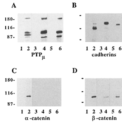
Figure 3. PTP \mu , cadherins, \alpha - and \beta -catenin are associated in lung, heart, and brain tissue. This figure represents IP immunoblots from lysates of lung (lanes 1 and 2), heart (lanes 3 and 4) and brain (lanes 5 and 6). Lanes 1, 3, and 5 are immunoprecipitates using mouse IgG. Lanes 2, 4, and 6 are immunoprecipitates using antibody (BK2) to the extracellular domain of PTP \mu . The immunoblot in A was probed with antibody (SK15) to PTP \mu . The immunoblot in B was probed with antibody (RPan) to cadherin. C and D were probed with antibodies (RAC and RBC) to \alpha - and \beta -catenin, respectively. PTP \mu was found associated with cadherins and \beta -catenin in all three tissues. \alpha -catenin was only observed to coprecipitate with PTP \mu in lung tissue.
