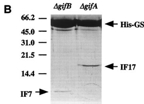
FIG. 2. (A) In vivo ammonium-dependent GS inactivation in Synechocystis wt and Δ gifA , Δ gifB , and Δ gifAgifB mutants. wt, Δ gifA , Δ gifB , and Δ gifAgifB Synechocystis cells were grown in BG11 medium by using nitrate as nitrogen source. Ammonium chloride (5 mM) was added at t = 0, and GS biosynthetic activity was determined, in situ , at the indicated times. (B) Δ gifA and Δ gifB Synechocystis HTGS1 cells were grown in BG11 medium and treated with 5 mM of ammonium chloride for 2 h. His-GS was purified by Ni-affinity chromatography and subjected to SDS/PAGE and Coomassie blue staining.
