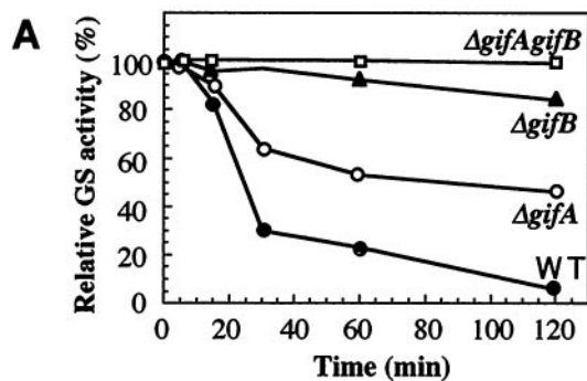
FIG. 2. (A) In vivo ammonium-dependent GS inactivation in Synechocystis wt and Δ gifA , Δ gifB , and Δ gifAgifB mutants. wt, Δ gifA , Δ gifB , and Δ gifAgifB Synechocystis cells were grown in BG11 medium by using nitrate as nitrogen source. Ammonium chloride (5 mM) was added at t = 0, and GS biosynthetic activity was determined, in situ , at the indicated times. (B) Δ gifA and Δ gifB Synechocystis HTGS1 cells were grown in BG11 medium and treated with 5 mM of ammonium chloride for 2 h. His-GS was purified by Ni-affinity chromatography and subjected to SDS/PAGE and Coomassie blue staining.
