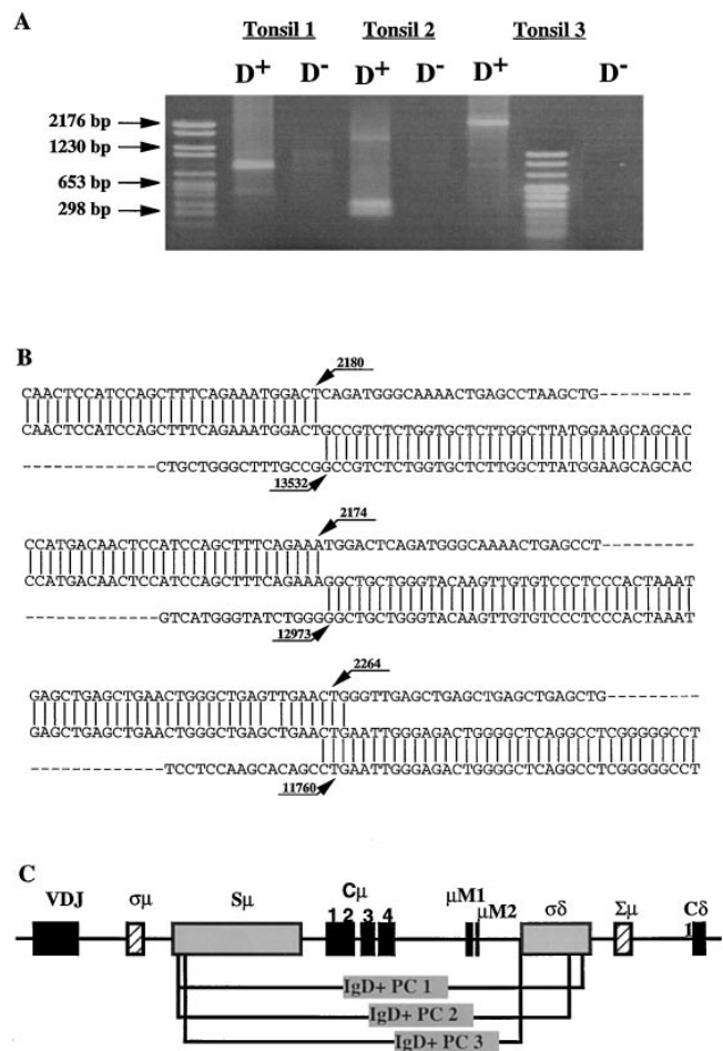
Figure 5. C \mu -C \delta switch recombinations in IgD + plasma cells of three tonsil samples. (A): PCR amplification and S \mu - \sigma / \delta recombinations of genomic DNA from IgD + (lanes D + ) and IgD - (lanes D - ) plasma cells. (B) DNA sequences of S \mu - \sigma / \delta junctional regions from IgD + plasma cells. Upper strings , germline sequences of the S \mu region; lower strings , germline sequences of the \sigma / \mu - \sigma / \delta intron. The central string represents the sequences of cloned PCR products. Homologous nucleotides are linked by vertical bars. Arrowed figures , the base numbers, base No. 1 being the first 3' of the VDJ region. (C) Schematic representation of the break points.
