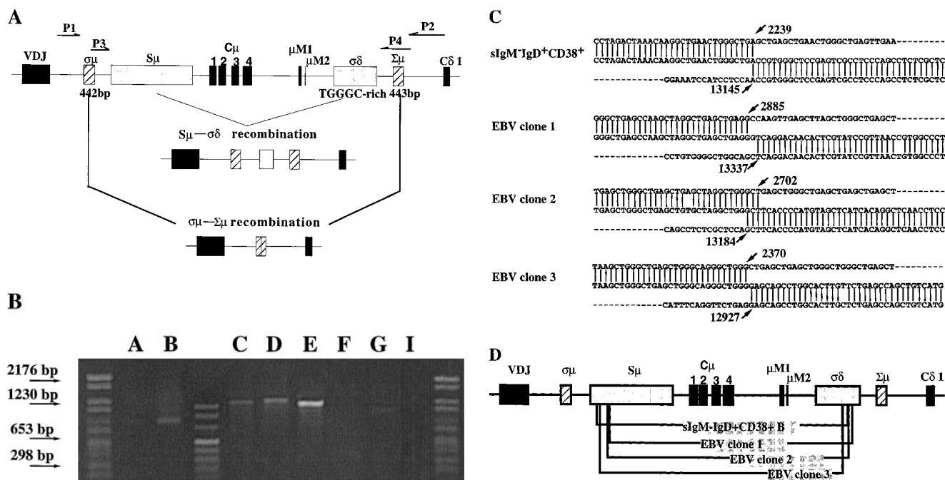
Figure 1. C\mu - C\delta switch recombinations in IgM - IgD + CD38 + GC B cells. (A) Schematic representation of the S\mu - \sigma\delta and \sigma\mu - \Sigma\mu recombinations (14–16). (B) PCR amplification of S\mu - \sigma\delta recombination. Lane A, IgM - IgD + CD38 + GC founder cells; lane B, IgM - IgD + CD38 + GC B cells; lanes C, D, and E, EBV clones from IgM - IgD + CD38 + cells; lanes F, G, and I, EBV clones from IgM + IgD + CD38 + cells. (C) DNA sequences of S\mu - \sigma\delta junctional regions from IgM - IgD + CD38 + cells. Upper strings , germline sequences of the S\mu region; lower strings , germline sequences of the \sigma\mu - \sigma\delta intron. The central string represents the sequences of cloned PCR products. Homologous nucleotides are linked by vertical bars. Arrowed figures , base numbers, base No. 1 being the first 3' of the VDJ region. (D) Schematic representation of the break points.
