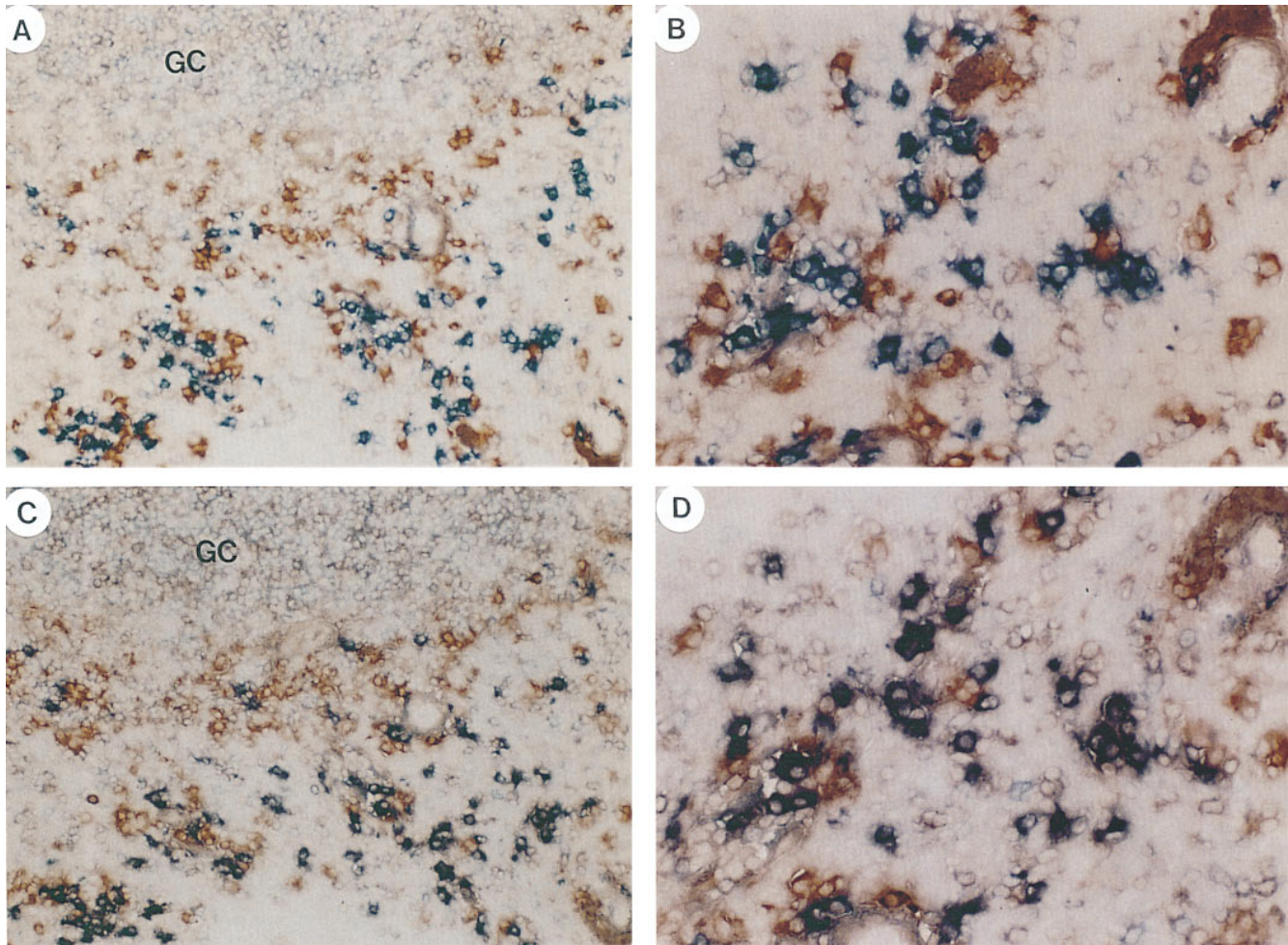
Figure 6. Ig light chain expression by tonsillar plasma cells. (A and B) Double blue anti-IgD and red anti-Ig \kappa staining showing many single stained blue Ig \kappa - IgD + plasma cells and a few double stained purple Ig \kappa + IgD + plasma cells. (C and D) Double blue anti-IgD and red anti-Ig \lambda staining on a serial section, showing many double stained Ig \lambda + IgD + plasma cells in purple and a few Ig \lambda - IgD + plasma cells single stained in blue. Original magnifications: 100 (A and C) and 400 (B and D).
