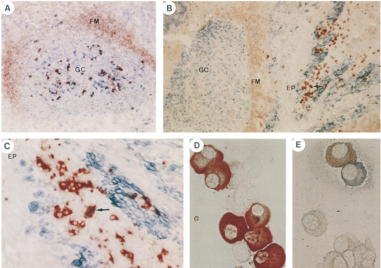
Figure 3. Ig heavy chain expression by tonsillar plasma cells. Immunoenzymatic staining of tonsillar tissue sections (A, B, and C) or plasma cell cytospin preparations (D and E). (A) Double red anti-IgD and blue anti-CD38 staining showing purple IgD + plasma cell within a GC and red IgD + follicular mantle (FM) B cells. Original magnification: 400. (B and C) Double red anti-IgD and blue anti-Ki67 staining showing red IgD 2+ plasma cells under the tonsillar epithelium (EP). Original magnifications are 100 (B) and 400 (C). (D) Single red anti-IgD staining showing IgD + plasma cells among purified tonsillar plasma cells. Original magnification: 1,000. (E): Double blue anti-IgD and red anti-IgM staining showing exclusive expression by plasma cells of each isotype. Original magnification: 1,000.
