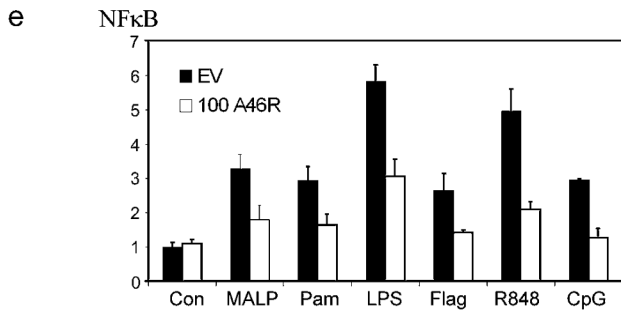
Figure 2. A46R associates with MyD88 and blocks MyD88-dependent signaling. (a) Alignment of A46R with human TIR domains. The conserved motifs Box 1, Box 2, and Box 3 are indicated by a solid line. The eight differences between VV and variola virus A46R sequences are indicated by an asterisk. For A46R, amino acids 35–238 are shown. (b) HEK 293T cells were transfected with A46R and AU1-MyD88 (left) or Flag-TRAF2 (right) as indicated. After 24 h, lysates were subject to immunoprecipitation, SDS-PAGE, and immunoblotting with the indicated antibodies. (c) HEK 293T cells were transfected with 8 \mu g AU1-MyD88 (top) or Flag-TRAF2 (bottom). After 24 h, lysates were incubated with GST alone (lane 2) or GST-A46R (lane 3), and together with whole cell lysates (lane 1) were analyzed by SDS-PAGE and immunoblotting with the indicated antibodies. (d) HEK 293
