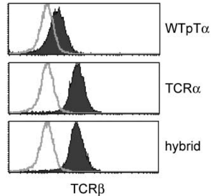
Figure 6. Influence of the extracellular region of TCRα on the behavior of the hybrid molecule. TCRβ levels on the surface of the 58α -β+ T cell hybridoma are influenced by the second extracellular domain TCRα. 58α -β+ hybridoma cells were infected with retroviruses encoding WTpTα, TCRα, or TCRα/pTα hybrid molecules, followed by an internal ribosomal entry site and enhanced green fluorescent protein (EGFP). Infected cells were identified by EGFP expression. Shaded histograms represent TCRβ surface staining on cells infected with retroviruses expressing WTpTα, TCRα, or TCRα/pTα hybrid molecules. The overlay represents TCRβ staining on cells infected with a control retrovirus expressing EGFP alone. The 58α -β+ T cell hybridoma is a variant of the DO-11.10.7 mouse T cell hybridoma that does not express functional TCRβ or TCRα chains (28).
