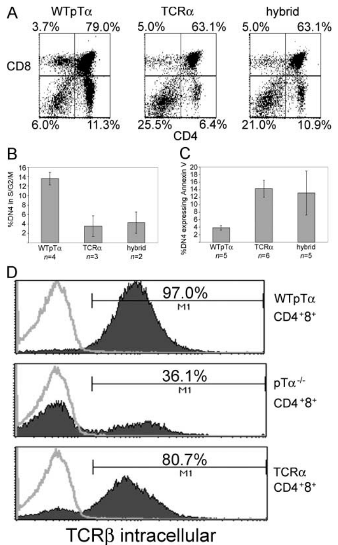
Figure 2. Defective differentiation, cell cycle entry, and survival of thymocytes expressing TCR \alpha and hybrid transgenes. (A) Dot plots depict the CD4 versus CD8 profile of a minimum of five 3–5-wk-old mice of each transgenic construct. Multiple founders were analyzed. (B) Percentage of sorted Gr-1 - Ter-119 - Dx5 - CD19 - TCR \gamma\delta - CD4 - CD8 - CD25 + CD44 - (DN4) thymocytes in the S/G2/M phases of the cell cycle. DNA content was analyzed by propidium iodide staining. (C) Percentage of DN4 thymocytes expressing externalized phosphatidyl serine apoptosis marker as revealed by staining with Annexin V. (D) Percentage of CD4 + 8 + thymocytes expressing intracellular TCR \beta (shaded histogram). Overlay represents intracellular staining with isotype-matched control antibody.
