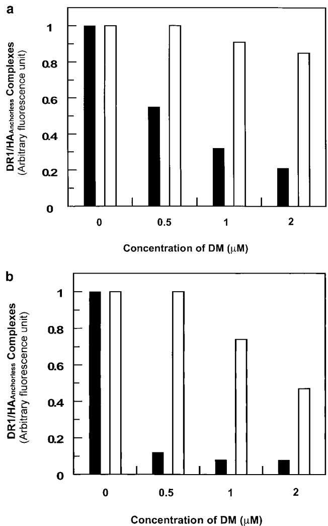
Figure 3. The effects of DM on dissociation of DR1-peptide complex in pH 6.0. 2.4 \mu M wtDR1 (black bars) and DR1 _{\beta G86Y} (white bars) in complex with FITC-HA _{Anchorless} were incubated with DM (citrate buffer, pH 6.0) for 20 min (a) or 40 min (b), and dissociation of the complexes was measured. At the physiological ratio of 1:5 DM/DR (reference 45), DM did not affect dissociation of the DR1 _{\beta G86Y} -HA _{Anchorless} complexes, whereas at higher molar ratios, up to 50% of the complexes dissociated after 40 min of incubation.
