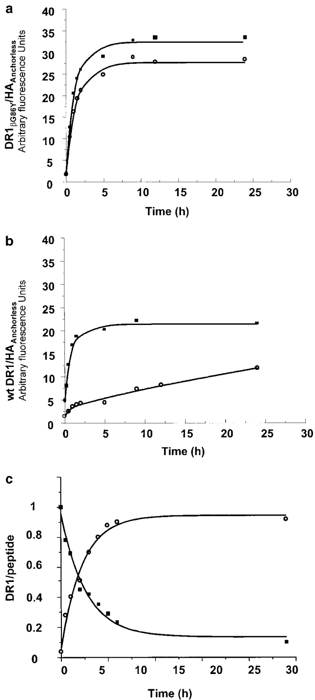
Figure 2. The effects of DM on the generation of receptive DR1. (a and b) The effects of DM on the binding of HA _{Anchorless} peptide to wt and DR1 _{\beta G86Y} . 2.4 \mu M DR1 _{\beta G86Y} (a) and wt (b) were incubated with 100 \mu M FITC-HA _{Anchorless} peptide for various times in the absence (○) and presence (■) of DM (1 \mu M, 0.15 M citrate phosphate buffer, pH 6.0, at 37°C). The calculated rates for peptide binding to DR1 _{\beta G86Y} , in the absence and presence of DM, to wtDR1 in the presence of DM, and to the receptive wtDR1, were all very similar and ranged between 0.47 and 0.61 s^{-1}\mu M^{-1} . (c) The kinetics of HA peptide binding to dissociating DR1-HA _{Anchorless} complex. 50 \mu M FITC-HA was incubated with 2.4 \mu M DR1-AMCA-HA _{Anchorless} complex (isolated by size-exclusion chromatography, citrate buffer, pH 6.0) for various times at 37°C. The unbound peptides were then removed by Sephadex G-50 spin columns in PBS. Samples were read at two wavelengths of 345 (AMCA) and 514 nm (fluorescein). The dissociation data (■) were fit to a single exponential decay curve. The HA association (○) data were fit to a single exponential binding curve.
