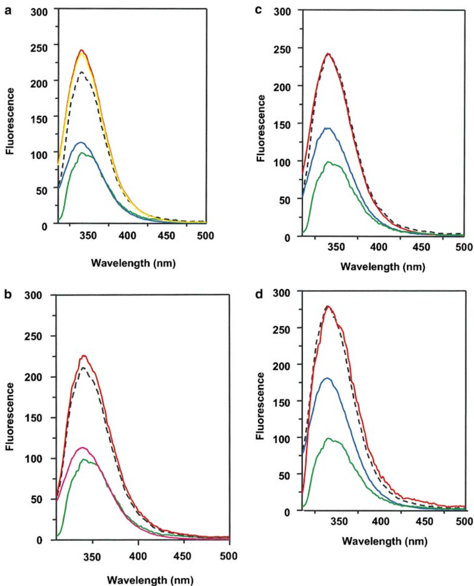
Figure 6. Interaction between DM and DR1 involves intrinsic tryptophan fluorescence changes. Intrinsic tryptophan fluorescence of DM interacting with empty wtDR1 (a), wtDR1–HA Ancorless (b), empty DR1 B86Y (c), and wtDR1–HA (d) complexes. DM and DR1 molecules (in citrate buffer, pH 6.0) were mixed and tryptophan fluorescence was measured immediately (red) and 1 h after mixing (yellow) for wtDR1 plus DM sample. The intrinsic tryptophans of each sample were excited at 295 nm to minimize the interference of tyrosine fluorescence and the emission spectra were obtained from 310 to 500 nm. Measurements for DM alone (green), DR alone (blue), and the mathematical sum (dashed line) are shown. The average fluorescence intensities from two separate measurements are plotted.
