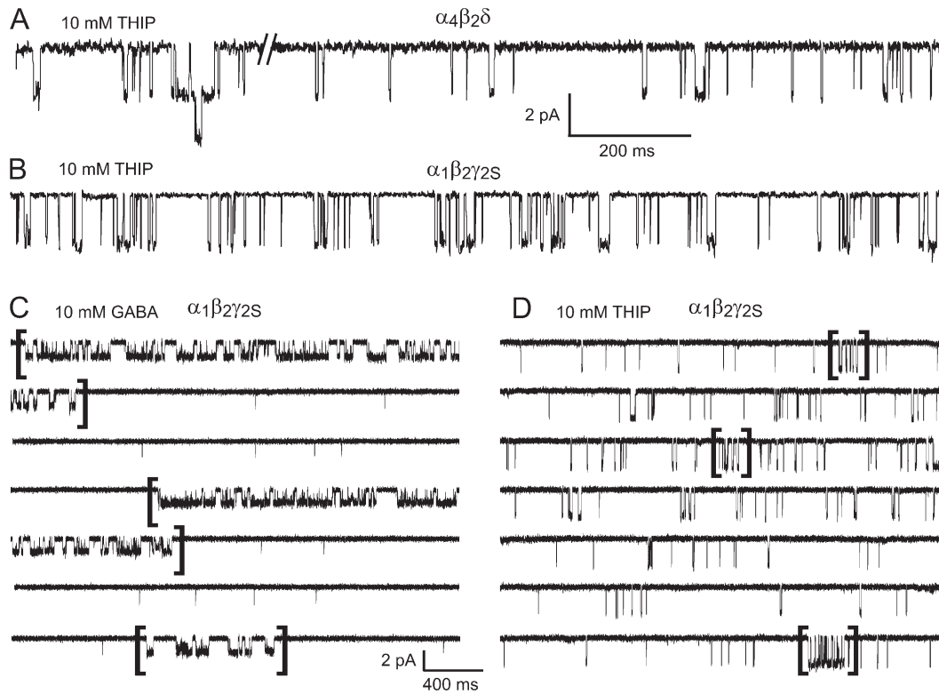
Figure 4. Single channel activity is agonist dependent in \alpha_4\beta_2\delta and \alpha_1\beta_2\gamma_2s GABA A Rs. Single channel recordings from patches expressing \alpha_4\beta_2\delta GABA A Rs (A) and \alpha_1\beta_2\gamma_2s GABA A Rs (B) in response to THIP. Bursts from both channel types were of relatively short duration (average burst duration <50 ms) and showed no apparent modal bursting. The intraburst open probability ( P_O ) was also similar for both channels, being \sim 0.4 – 0.5 . \alpha_1\beta_2\gamma_2s GABA A Rs typically opened more frequently than \alpha_4\beta_2\delta GABA A Rs. Continuous 3-s sweeps of single channel recordings from the same patch expressing \alpha_1\beta_2\gamma_2s GABA A Rs in response to GABA (C) and THIP (D). Note the absence of long quiescent periods, the larger current amplitude, and shorter clusters of activity (in square parentheses) in the presence of THIP. Currents were filtered to 2 kHz for display purposes.
