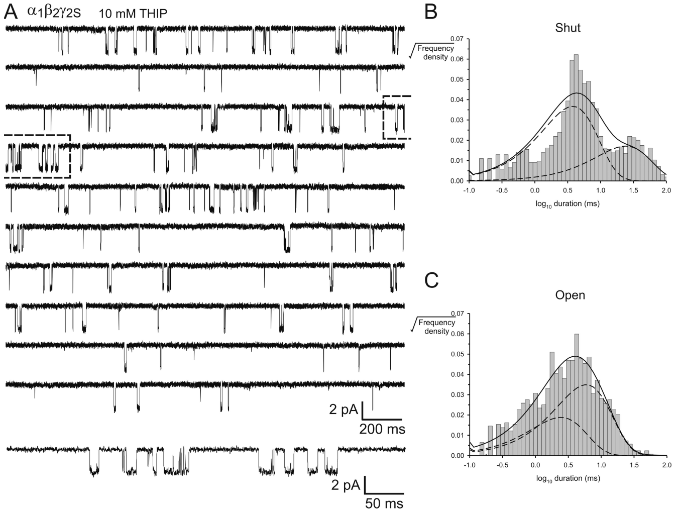
Figure 7. Burst analysis of THIP-activated \alpha_1\beta_2\gamma_{2S} GABA A Rs. (A) Continuous, 2-s sweeps of single channel activity recorded from a patch expressing \alpha_1\beta_2\gamma_{2S} GABA A R in response to 10 mM THIP. The cluster enclosed in the box is expanded below. (B) Dwell time histogram of apparent shut intervals and (C) dwell time histogram of apparent open intervals for the activity shown in A. Distributions were fit with a mixture of exponential probability density functions (dark lines). The individual components are shown as broken lines. The analysis revealed two shut and two open components for this activity. Currents were filtered to 2 kHz for display purposes.
