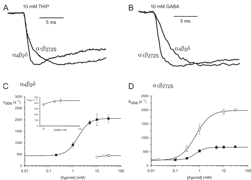
Figure 2. Current activation rates for \alpha_4\beta_2\delta and \alpha_1\beta_2\gamma_{2S} GABA A Rs in response to THIP and GABA. (A) The activation phase of currents mediated by \alpha_4\beta_2\delta and \alpha_1\beta_2\gamma_{2S} GABA A Rs in response to fast agonist application of THIP, showing that THIP activates \alpha_4\beta_2\delta GABA A Rs more rapidly. (B) The activation phase of currents for \alpha_4\beta_2\delta and \alpha_1\beta_2\gamma_{2S} GABA A Rs in response to fast application of GABA, showing that \alpha_1\beta_2\gamma_{2S} GABA A Rs activate more rapidly. (C) Plot of activation rate constant ( k_{\text{obs}} ) versus [agonist] for \alpha_4\beta_2\delta GABA A Rs. The plot for GABA-gated activation is shown on an expanded scale (inset). (D) Plot of activation rate constant ( k_{\text{obs}} ) versus [agonist] for \alpha_1\beta_2\gamma_{2S} GABA A Rs. The data points were fitted to a modified form of the Hill equation (see Materials and methods). The parameters of the fit are shown in Table I. THIP, black symbols; GABA, white symbols.
