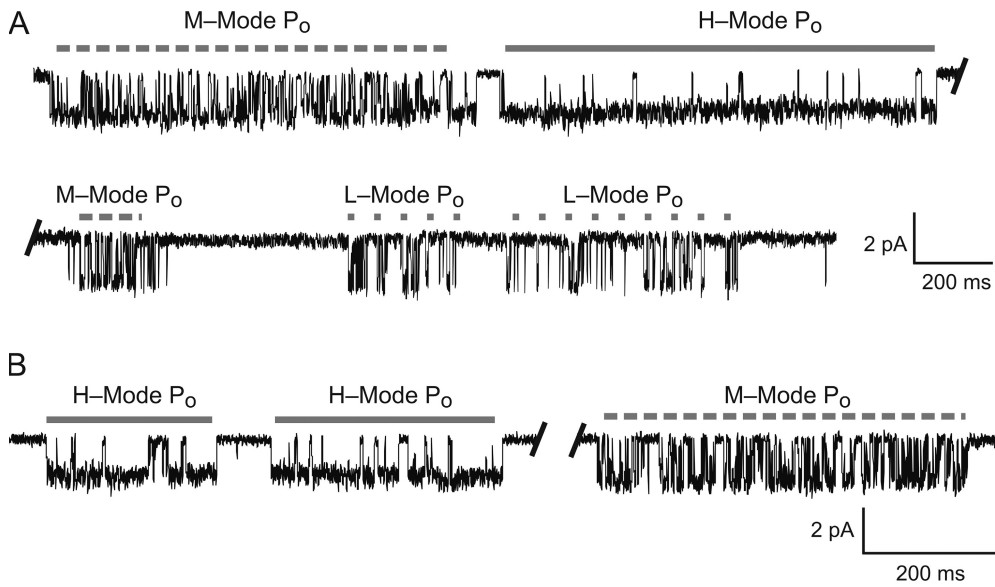
Figure 5. GABA elicits bursting modes in \alpha_1\beta_2\gamma_{25} GABA A Rs. (A) A patch exhibiting medium mode (M-Mode P O ), high mode (H-Mode P O ), and low mode (L-Mode P O ) clusters in the presence of 10 mM GABA. (B) Another patch exhibiting only the H-Mode P O and M-Mode P O gating patterns. Currents were filtered to 2 kHz for display purposes.
