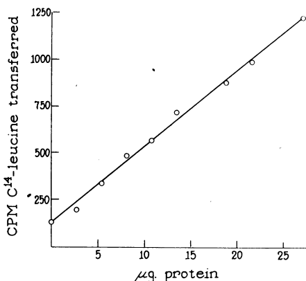
FIG. 2.—Concentration curve of transfer factor. The incubation mixture consisted of washed ribosomes (1.3 mg protein), 0.31 mg of sRNA charged with amino acids including 6660 cpm C^{14} -leucine ( 1.45 \times 10^7 cpm/ \mu mole), 0.0006 M GTP, 0.01 M PEP, 30 \mu g/ml PEP-kinase, 0.01 M GSH, 0.013 M MgCl_2 , 0.03 M KCl, 0.05 M Tris HCl pH 7.4, and purified transfer factor as noted, in a volume of 0.50 ml. After 5 minutes at 30^\circ , 5 per cent TCA was added, the precipitate extracted with 5 per cent TCA at 90^\circ for 15 minutes, washed twice with TCA, once with 1:1 ethanol-ether, and counted in a windowless gas flow counter.
