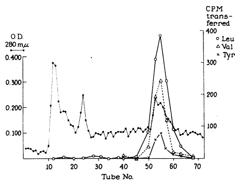
FIG. 1.—DEAE-cellulose column chromatogram of transfer factor. Application of 55 mg of the ammonium sulfate fraction was made to a 1.3 \times 40 cm column equilibrated at 4^\circ with 0.010 M potassium phosphate pH 7.4; 100 ml of 0.10 M potassium phosphate, pH 7.4, was passed through and a linear gradient of the same pH from 0.10 M to 0.25 M potassium phosphate started after tube 17. All buffers contained 0.004 M mercaptoethanol. Fraction volumes of 7 ml were collected and assayed for transfer factor with the labelled aminoacyl-sRNA's noted. Assay conditions were the same as given in Fig. 2, except as follows: with leucine and valine, 1.4 mg of ribosomal protein, 0.24 mg of sRNA (5000 cpm C^{14} -leucine, or 4040 cpm C^{14} -valine containing 1.23 \times 10^7 cpm/ \mu mole); with tyrosine, 3.5 mg of ribosomal protein, 0.57 mg of sRNA (1700 cpm C^{14} -tyrosine containing 5.2 \times 10^6 cpm/ \mu mole).
