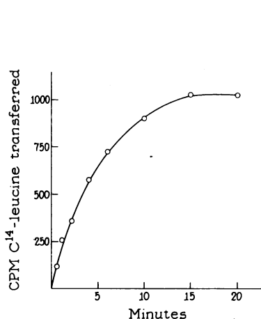
FIG. 4.—Time curve of leucine transfer from sRNA to protein. Incubation conditions as given in Fig. 2, except that the volume was 6.0 ml and contained ribosomes (20 mg protein), 7.2 mg of transfer factor, 5.0 mg of sRNA charged with amino acids including 51,000 cpm C^{14} -leucine. At each time point, 0.50 ml was pipetted into 5 per cent TCA and the precipitate treated as described in Fig. 2.
