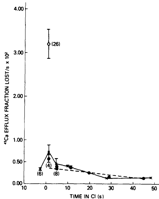
FIGURE 7. The rate of 45 Ca loss to the bath with EGTA present initially; 5 mM EGTA was applied just preceding the Cl stimulus (×) or simultaneously (⊗). Data are plotted as in Fig. 6. (○) shows the initial 45 Ca efflux in Cl in the absence of EGTA (pooled mean ± SEM for all data on completed and interrupted responses). The unstimulated 45 Ca efflux in propionate solution with 5 mM EGTA is shown by the dashed line (●) (mean ± SEM of pooled data shown in Figs. 1 and 2).
