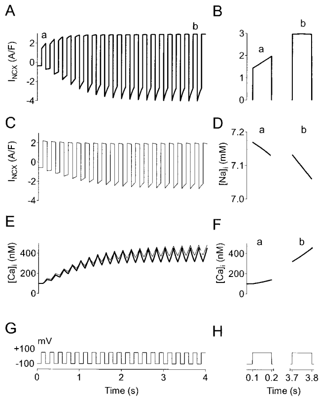
FIGURE 8. Computer simulations based on model in Fig. 1. (A, bold trace) I_{\text{NCX}} with Ca activation (Eq. 1, K_{\text{mCaAct}} = 125 nM). Both outward and inward I_{\text{NCX}} grow as [\text{Ca}]_i increases in response to alternating protocol. (B) Outward I_{\text{NCX}} during single pulses, early (a) and late (b) of A. (C, thin trace) I_{\text{NCX}} (Eq. 1 with allosteric factor omitted). Without Ca activation, outward I_{\text{NCX}} declines slightly while inward I_{\text{NCX}} increases less dramatically. (D) [\text{Na}]_i time course for pulses B (a and b). (E) [\text{Ca}]_i time course with (bold trace) and without (thin trace) Ca activation. (F) [\text{Ca}]_i time course for pulses B (a and b). (G) Voltage protocol was identical for all simulations. (H) Voltage for pulses B (a and b). In all simulations, Ca background leak density ( G_{\text{CaBkg}} ) was adjusted to give initial resting [\text{Ca}]_i = 100 nM at -100 mV. Simulation parameters based on fits to the ferret data are given in Table II. Other parameters not based on our experiments are given in MATERIALS AND METHODS.
