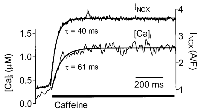
FIGURE 9. Rapid time course of development of Ca activation in ferret myocyte. Caffeine was applied at +100 mV to cause rapid increase in [\text{Ca}]_i . There was no apparent delay between the activation of outward I_{\text{NCX}} and the rise in [\text{Ca}]_i . Solutions were identical to those described in MATERIALS AND METHODS, but pretreatment with thapsigargin- and caffeine-containing solutions was omitted.
