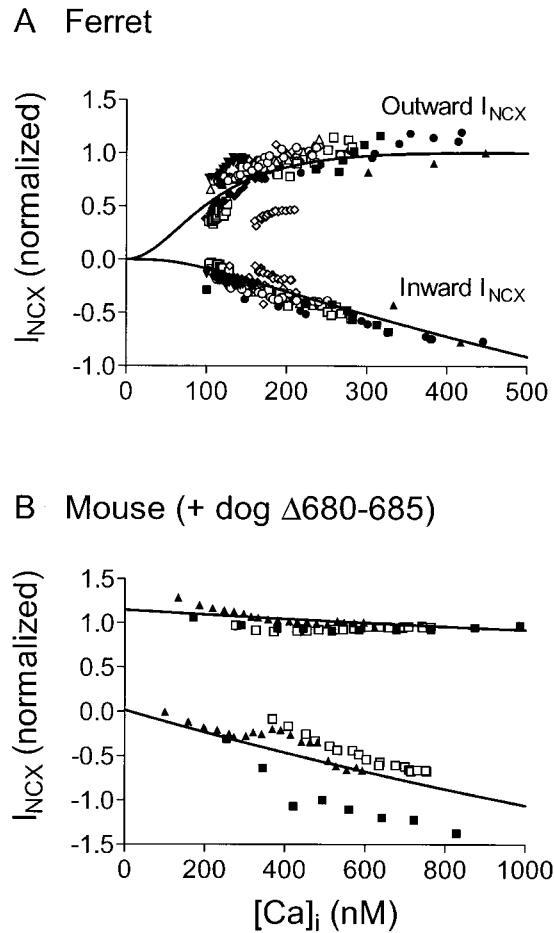
FIGURE 5. I_{NCX} versus [Ca]_i fit to Eq. 1. (A) Solid lines show outward and inward I_{NCX} predicted from fits to the ferret data including the allosteric factor ( K_{mCaAct} = 125 nM). Data of all 14 cells were less well fit ( P < 0.05 ) when the allosteric factor was not included. (B) Solid lines show outward and inward I_{NCX} predicted from fits to data of mouse myocytes overexpressing \Delta 680-685 canine NCX1 without the allosteric factor. Including the allosteric factor did not improve the fits. Each symbol in A and B represents time-averaged I_{NCX} during a particular voltage step at the corresponding averaged [Ca]_i . For clarity, the figure shows data normalized to the fit predictions at [Ca]_i = 500 nM in A and [Ca]_i = 1,000 nM in B.
