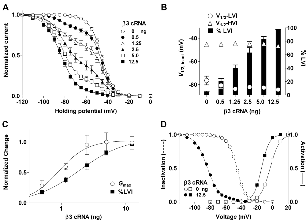
FIGURE 3. The \beta 3 -induced hyperpolarizing shift of the steady-state inactivation curves of N-type calcium channels is attributed to change in the proportion of two components of the curves. Oocytes were injected with cRNAs as shown in Fig. 2. (A) Steady-state inactivation for HPs of 3-min duration. Data are indicated as mean \pm SE ( n = 7 –15 from 3–7 frogs for each group). Note that HPs of 3 min did not induce maximal inactivation and therefore reflect “pseudo-steady-state” inactivation (compare Fig. 8). (B) Effects of the \beta 3 subunit on inactivation midpoints ( V_{1/2, \text{inact}} ) of LVI (open circle) and HVI (open triangle) and the proportion of LVI (%LVI; closed column). Plotted data were derived from the curve fitting in panel A and shown as mean \pm SE. (C) Difference in concentration dependency of the \beta 3 -induced enhancement of G_{\text{max}} and increase in the %LVI. Plotted data were derived from B and Fig. 2 C for %LVI and G_{\text{max}} at a HP of -120 mV, respectively. Data were normalized by dividing each value by the maximum value and are expressed as mean \pm SE. (D) No or little overlap of activation and inactivation curves seen in the presence or absence of \beta 3 . Plotted data were derived from panel A and Fig. 2 B.
