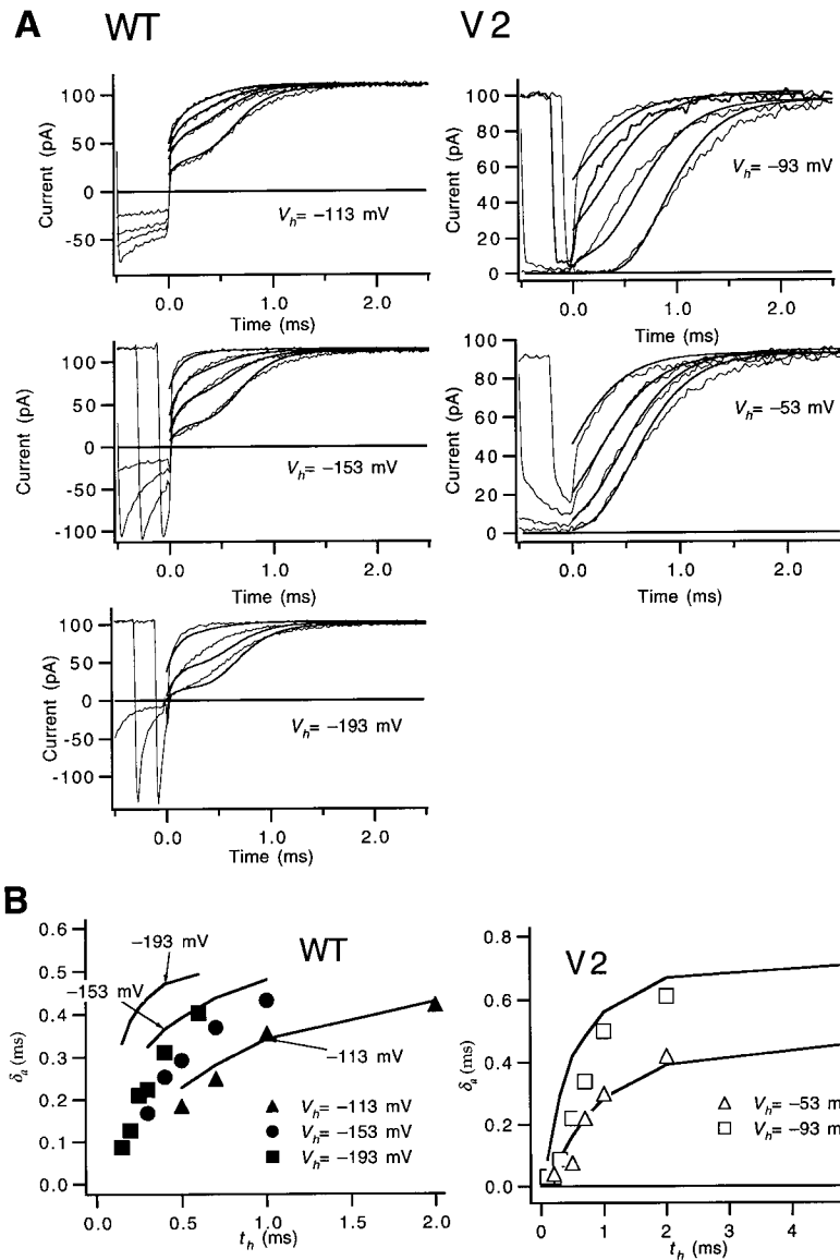
FIGURE 16. Scheme 3+2' accounts for some but not all of WT's and V2's reactivation time courses. (A) Selected WT and V2 reactivation time courses from Fig. 10 were fitted to Scheme 3+2'. Scheme 3+2' accounts for the reactivation time courses for the less negative V_h reasonably well, but fails to account for the reactivation time courses for the most negative V_h . In these simulations, for WT, the values of a_1 , a_2 , and a_3 were each increased by 20% compared with the values in Table III, and the values for \beta_{N-1}(0) and \beta_N(0) were 520 \text{ s}^{-1} and \beta_N = 280 \text{ s}^{-1} . For V2, \beta_N was changed to 1,100 \text{ s}^{-1} . (B) The same deviations in the fits are shown in a comparison of the \delta_a values that were derived from the measured and simulated currents in A. These discrepancies reflect the 20% increases in q_{b1} , q_{b2} , and q_{b3} , used to help achieve a sufficiently large total gating charge.
