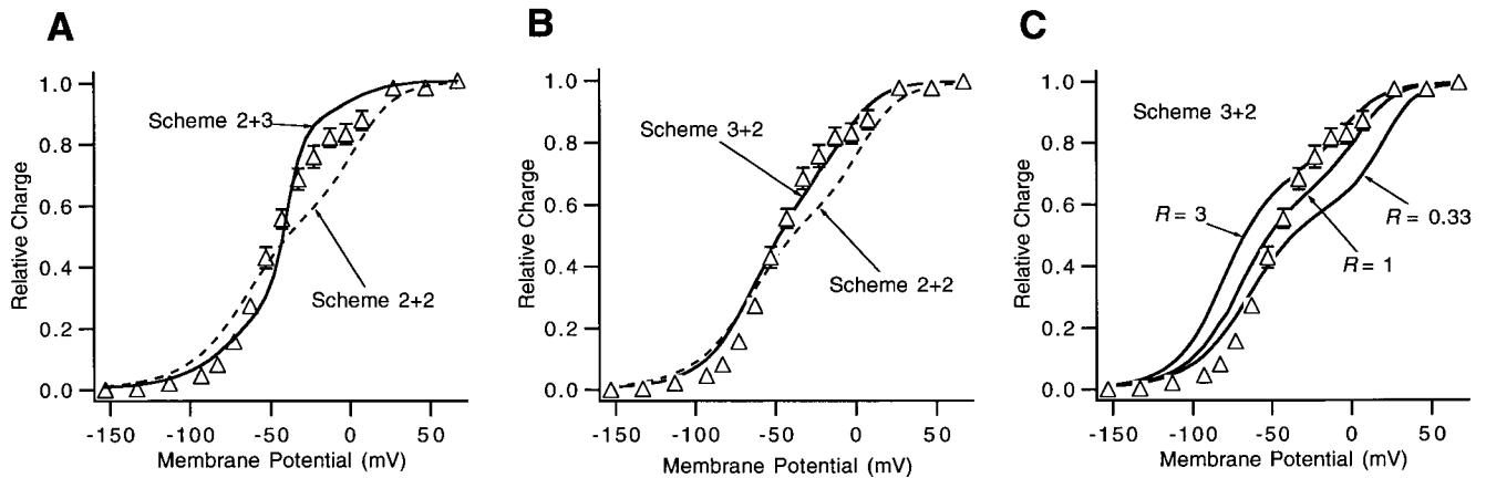
FIGURE 12. Constraints on how to add more transitions to Scheme 2+2' were provided by the shape of V2's Q - V relation. (A) V2's mean Q - V relation has been superimposed (solid curve) with predictions of Scheme 2+3', with the concerted transition in the third to last position having a valence of 3.5. This model steepens the Q - V relation compared with the predictions of Scheme 2+2' (dashed curve). However, it yields a Q - V relation that is too steep at voltages near -40 mV, while remaining too shallow at hyperpolarized voltages (near -80 mV). For the simulations, the parameter estimates for all but the large valenced transition were fixed to be the same as in Scheme 2+2'; the midpoint voltage of the new transition was varied to best account for V2's Q - V relation. (B) Scheme 3+2' performs better at steepening V2's Q - V relation across the entire voltage range. For these simulations, the parameter values for S_0 \leftrightarrow S_1 and S_1 \leftrightarrow S_2 were those given for the same transitions in Scheme 2+2' in Table II. For S_2 \leftrightarrow S_3 , we assigned a charge ( 0.88 e_0 ) that is one-fourth of the charge ( 3.5 e_0 ) assigned to the concerted transition in Scheme 2+3' in A. Its midpoint voltage was varied to yield the best fits of the data. (C) V2's Q - V relation was also used to obtain a rough estimate of the equilibrium constant for S_2 \leftrightarrow S_3 . Three different simulations of Scheme 3+2' are shown for different values of a factor R ( R = 3, 1 , and 0.33 ) that reflect the ratio of the equilibrium of S_2 \leftrightarrow S_3 versus that of S_1 \leftrightarrow S_2 . In these simulations, the charge associated with S_2 \leftrightarrow S_3 was assigned to be the same as that associated with S_1 \leftrightarrow S_2 , given in Table II.
