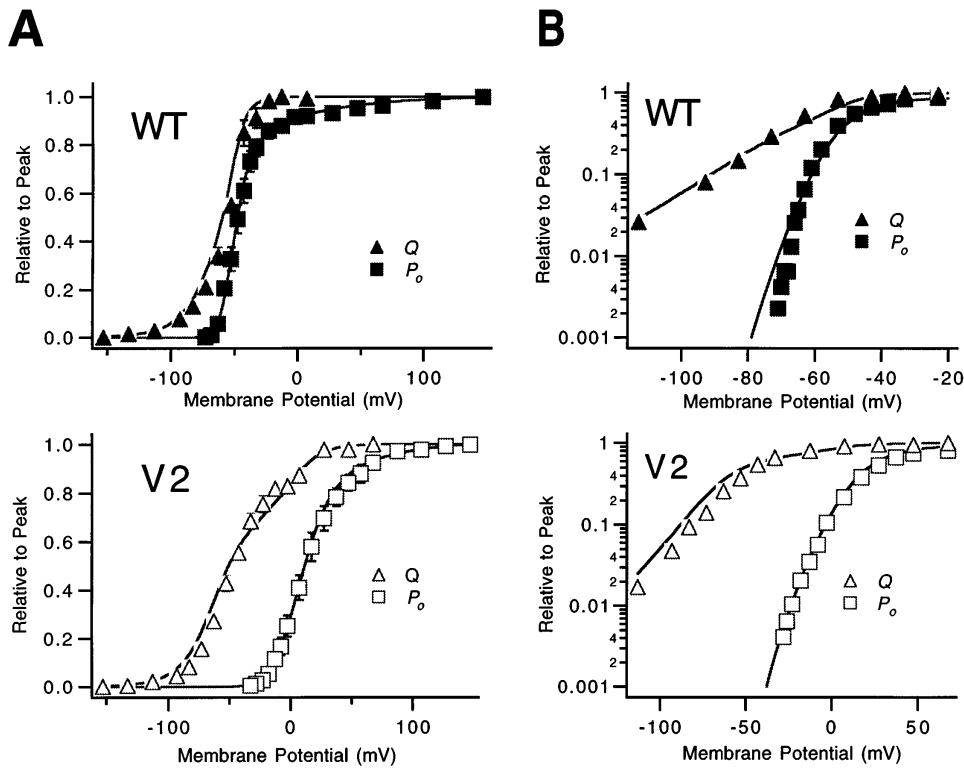
FIGURE 17. Scheme 3+2' performs much better than Scheme 2+2' at predicting certain features of WT's and V2's equilibrium voltage dependence of channel opening and charge movement, including the steepness of V2's Q - V relation and the voltage sensitivity of WT's P_o at low P_o . As in Fig. 11, plots are shown with ordinates that are linear (A) or log transformed (B).
