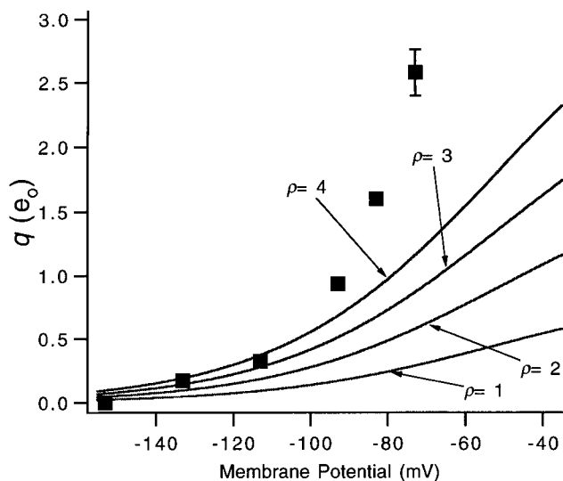
FIGURE 6. The magnitude of the average, absolute charge movement per channel at negative voltages was used to test the “ n^4 ” scheme as a model of the first gating transitions. The solid curves were computed from a model assuming a number p of equivalently acting subunits, for which the charge movement q is given by
