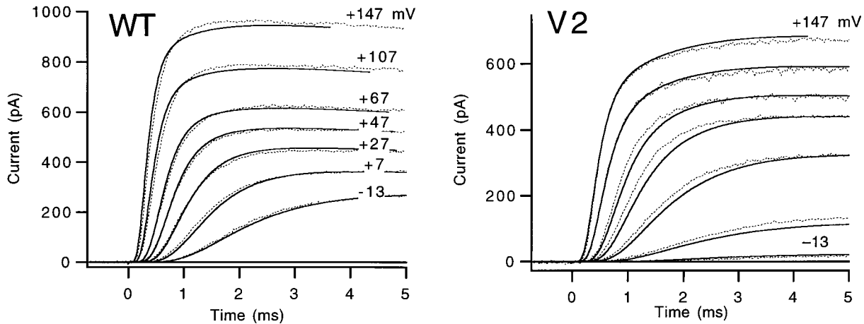
FIGURE 8. A modified version of Scheme 2+2' accounts for a slow component in the activation time course. In this model, the channel can enter the state C_{iN-1} from the last closed state C_{N-1} .
