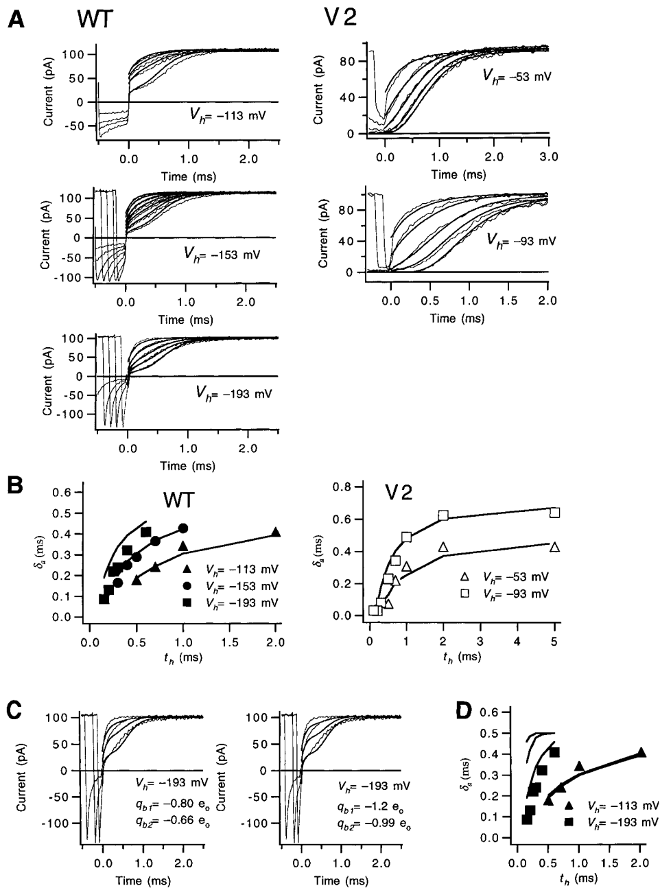
FIGURE 10. Fits of Scheme 2+2' to WT and V2 reactivation kinetics. (A) Scheme 2+2' accounts for WT and V2's reactivation time courses after hyperpolarizations of various amplitudes V_h (between -53 and -193 mV) and duration t_h . Test voltages were +37 and +67 mV for WT and V2, respectively. All of the displayed data come from the same WT and V2 patch recordings and correspond to the following t_h values. WT: for V_h = -113 mV, t_h = 0.5, 0.7, 1, and 2 ms; for V_h = -153 mV, t_h = 0.1, 0.2, 0.3, 0.4, 0.5, 0.7, and 1 ms; for V_h = -193 mV, t_h = 0.1, 0.2, 0.3, 0.4, and 0.6 ms. V2: for V_h = -53 mV, t_h = 0.2, 0.5, 1, 2, and 5 ms; for V_h = -93 mV, t_h = 0.1, 0.2, 0.5, 1, and 5 ms. In the simulations, for WT, a_1 and a_2 were each increased by 20% compared with the values in Table II, and the values for \beta_{N-1}(0) and \beta_N(0) were 520 and 280 s^{-1} . For V2, \beta_N was changed to 1,100 s^{-1} . Data are from patches w448 and v162. (B) Scheme 2+2' accounts for the delay \delta_a in WT and V2's reactivation time course for different V_h and t_h . The \delta_a values were derived from the measured and simulated currents from A. (C and D) WT's reactivation time courses were used to place constraints on the sizes of q_{b1} and q_{b2} . For reactivation time courses measured after V_h = -193 mV, values for q_{b1} and q_{b2} that are two or three times as large as the values in Table II predict a reactivation delay that is too long. In D, the three superimposed lines to the left of the squares reflect \delta_a values derived from simulated currents for the q_{b1} and q_{b2} values in Table II (the best fit) or q_{b1}
