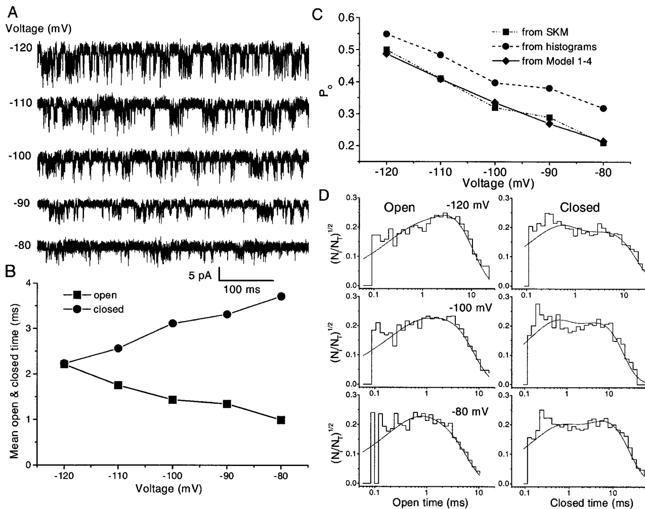
FIGURE 15. The effect of voltage on the single channel currents, mean open and closed times, and P_o . (A) Single-channel currents activated by 30 \mu M ATP were recorded at different membrane potentials. Other conditions were the same as in Fig. 4. All the current traces in this figure are from the same patch. The currents were idealized for further kinetic analysis after filtering at 5 kHz using a Gaussian digital filter. (B) Mean open and closed times extracted from the idealized currents as a function of voltage. (C) The probability of being open, P_o , as function of voltage calculated from idealized currents (■), all-points histograms (●), and the prediction by Fig. 13, Model 1-4 (◆). P_o from the histogram is slightly larger than that from idealized currents, indicating that some short-lived openings were missed during idealization. P_o predicted by Model 1-4 is close to P_o from idealized currents. (D) The closed and open time histograms at different voltages. The solid lines in the histograms are predicted probability density functions based on Model 1-4. N_i/N_T has the same meaning as in Fig. 10 C.
