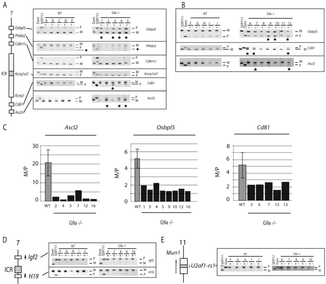
FIG. 2. Altered imprinted gene expression in G9a -/- placentas. (A) RT-PCR in the presence (+) or absence (-) of reverse transcriptase on (C57BL/6 × SDP711)F 1 placentas at 9.5 dpc (WT and G9a -/- ). In all panels, the first two lanes show control amplifications from C57BL/6 (Dom) and SDP711 WT placentas, respectively. Maternal (M) and paternal (P) specific bands are indicated. Asterisks indicate placentas in which the M/P ratio was different from that observed in the cohorts of WT placentas. In the Phlda2 analysis, the black dot indicates a secondary, maternal-specific band. (B) Loss of imprinting (asterisks) at Osbp15 , Cd81 , and Ascl2 was also observed in (SDP711 × C57BL/6)F 1 placentas. (C) M/P band intensity ratios. In each of the panels, the average ratio for all WT placentas analyzed is shown to the left. Examples of G9a -/- placentas that were below this range for Ascl2 , Osbp15 , or CD81 are shown to the right. In the G9a -/- placentas, M/P ratios were significantly lower than in WT placentas for Ascl2 (mean, 2.3 versus 5.2; P < 0.0001) and Osbp15 (mean, 2.3 versus 5.2; P < 0.00001). For Cd81 , the means were not different between the WT and G9a -/- mice (5.2 versus 8.4; P = 0.014). (D) Unaltered allelic expression of the Igf2 and H19 genes in G9a -/- placentas. (E) Unaltered paternal expression of the U2af1-rs1 gene.
