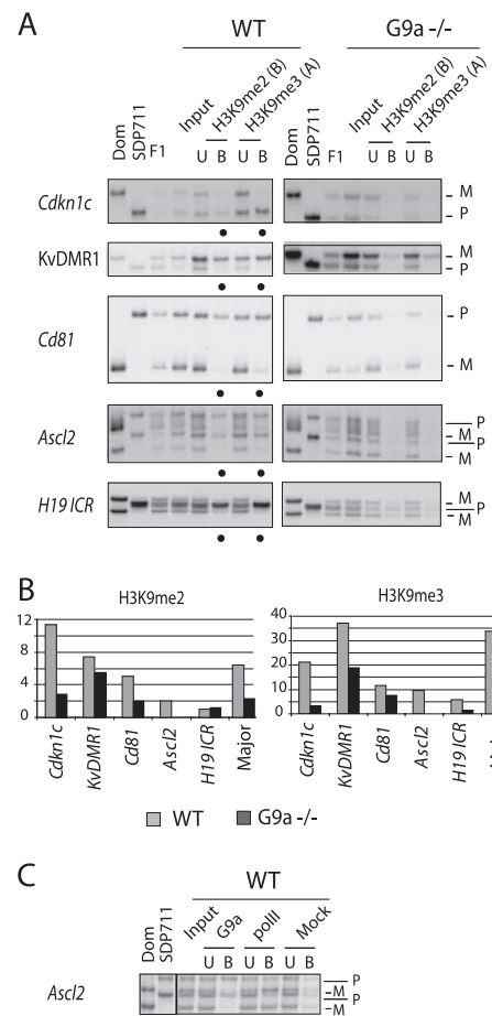
FIG. 4. Kcnq1 domain genes have reduced H3K9me2 and H3K9me3 in the absence of G9a . (A) ChIP was performed concomitantly on limited numbers of G9a -/- and WT placentas (at 9.5 dpc), using the same reagents. Chromatin was precipitated with antisera against H3K9me2 and H3K9me3. PCR was performed on antibody-bound (B) and unbound (U) fractions, followed by SSCP-based discrimination of the maternal (M) and paternal (P) alleles (for the precise location of primers, see Table S3 in the supplemental material). In all panels, the first four lanes show amplifications from C57BL/6 (Dom), SDP711, and (C57BL/6 × SDP711)F 1 (F1) genomic DNAs and from the used input chromatin (input). Black dots indicate allelic ratios which are >2 (after correction for the ratio in the input chromatin). (B) Levels of precipitation are presented as the enrichment over that of a mock precipitation with an unrelated IgG antiserum. In terms of percentage of input chromatin that was precipitated, this corresponds to 6% for H3Kme2 at Cdkn1c and 32% for H3K9me3 at the KvDMR1. (C) ChIP on fixed placental chromatin (WT). The first three lanes show control amplifications from C57BL/6 (Dom), SD7P711, and input chromatin, respectively. The allelic enrichment is marked by black dots when it was >2. Association of G9a was detected on the repressed paternal allele of Ascl2 ; RNA Pol II is associated with the active maternal allele.
