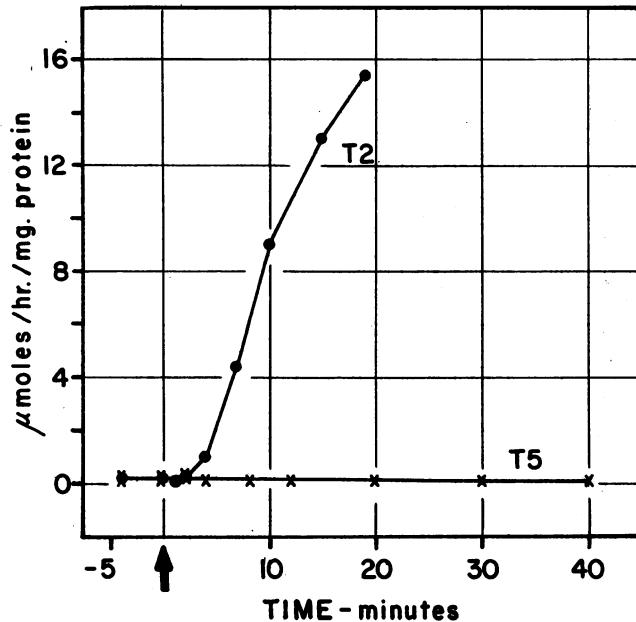
FIG. 3.—dCTPase levels before and after infection with phage T2 or T5. The arrow indicates the start of infection ("zero minutes," see Method I). The incubation mixtures (0.25 ml) contained: 6.0 \mu moles of dCTP labeled with P 32 in the terminal pyrophosphate group ( 10^3 cpm per \mu mole), glycine buffer, pH 9.2 (0.04 M), MgCl 2 (0.008 M), 2-mercaptoethanol (0.01 M) and a quantity of extract containing about 0.3 \mu g of protein. After 20 min of incubation at 37°, the reaction was terminated by adding 0.5 ml of 0.1 N HCl, followed by 0.2 ml of a mixture (containing per ml: 5 mg of crystalline bovine serum albumin, 25 \mu moles of sodium pyrophosphate and 25 \mu moles of potassium phosphate, pH 7), and 0.1 ml of a Norit suspension (20 per cent packed volume). The Norit was removed by centrifugation and the supernatant fluid was assayed for radioactivity.
