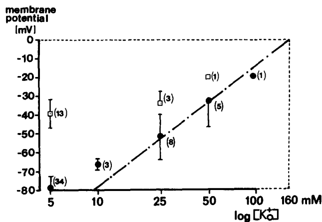
FIGURE 10. Dependence of membrane potential (ordinate) on the external concentration of \text{K}^+ represented in a semilogarithmic scale (abscissa). Filled circles are measurements in low \text{Ca}^{++} (2 mM) and open squares are measurements in high \text{Ca}^{++} (4 mM). Every point represents the mean and the vertical bars represent the standard deviation of several measurements obtained from records like those shown in Fig. 10. The number of measurements is in parentheses. The straight line has been drawn by eye and has a slope of \sim 61 mV per 10-fold increase in external \text{K}^+ concentration. The intercept of this line with the 0-mV axis gives an estimate of the internal concentration of \text{K}^+ .
