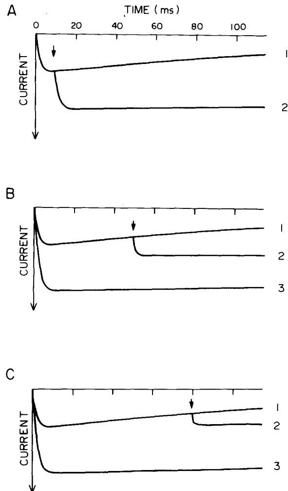
FIGURE 13. Simulations of the influence of flashes on the recovery from nifedipine blockade of the Ba^{2+} current. Rate constants are as described in the Appendix for the modulated receptor model. The lowest-amplitude trace in each case (labeled 1) represents the nifedipine-blocked current. Flashes (represented by arrows) were simulated during the traces labeled 2. The post-flash episodes (labeled 3) were simulated by assuming that the flash removed all the nifedipine from the channels and that, between traces 2 and 3, any inactivated channels were returned to the resting, closed state. When a flash is presented at the peak of the current ( A ), closed channels are unblocked. These channels open with the normal rate of current activation. In addition, after the flash, current decay slows because of the removal of nifedipine from the bath: open channel block is no longer evident. At longer times during a voltage step, the flash is less effective at recovering current amplitude, as shown in B and C . When the flash is delivered 50 ( B ) or 80 ( C ) ms into the step, blockade of both open and closed channels is relieved and there appear to be two components to the recovery.
