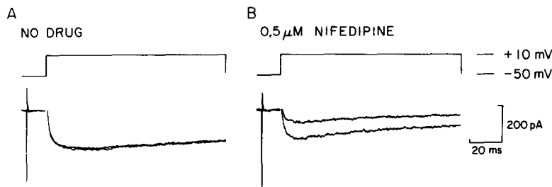
FIGURE 1. Photoremoval of nifedipine blockade of inward Ba^{2+} currents, which were elicited by stepping from a holding potential of -50 to +10 mV. Leakage currents have been subtracted. Each panel shows two superimposed consecutive current traces, evoked at an interval of 5 s. During the second sweep only, a flash was presented at the time indicated by the brief electrical artifact. In the absence of nifedipine (A), the flash had no effect on the current. In the presence of 0.5 \mu M nifedipine (B), the current was suppressed; in this case, the flash increased the current amplitude by reversing the nifedipine blockade.
