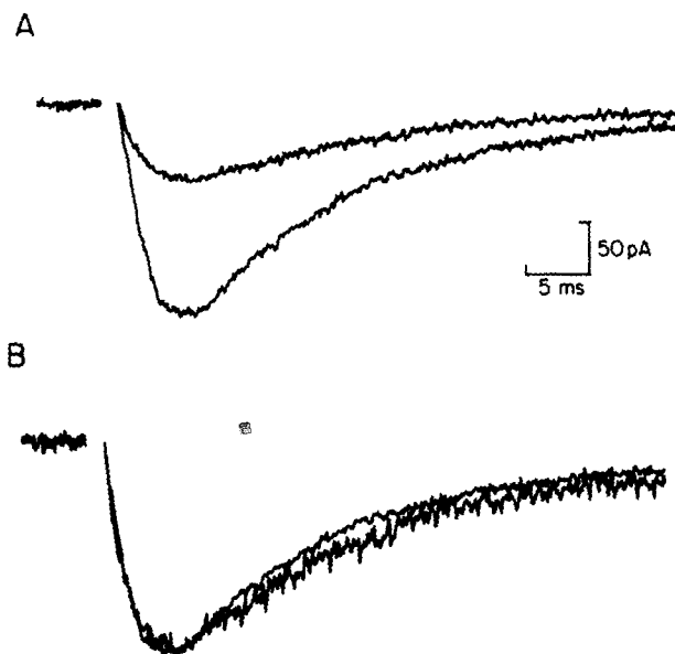
FIGURE 8. Influence of nifedipine on the waveform of \text{Ca}^{2+} currents. Nifedipine had little effect on the decay of I_{\text{Ca}} recorded in the presence of 10 \text{ mM Ca}^{2+} . During a 46-ms depolarizing step to +10 \text{ mV} from a holding potential of -50 \text{ mV} , the \text{Ca}^{2+} current amplitude decayed to \sim 90\% of the peak in the presence of 0.5 \mu\text{M} nifedipine (A, smaller trace). After a flash, although the peak amplitude of the current was enhanced, current decay was similar (A, larger trace). This is demonstrated more clearly when the currents are scaled and superimposed (B). Similar results were obtained at all nifedipine concentrations and all test potentials examined (data not shown).
