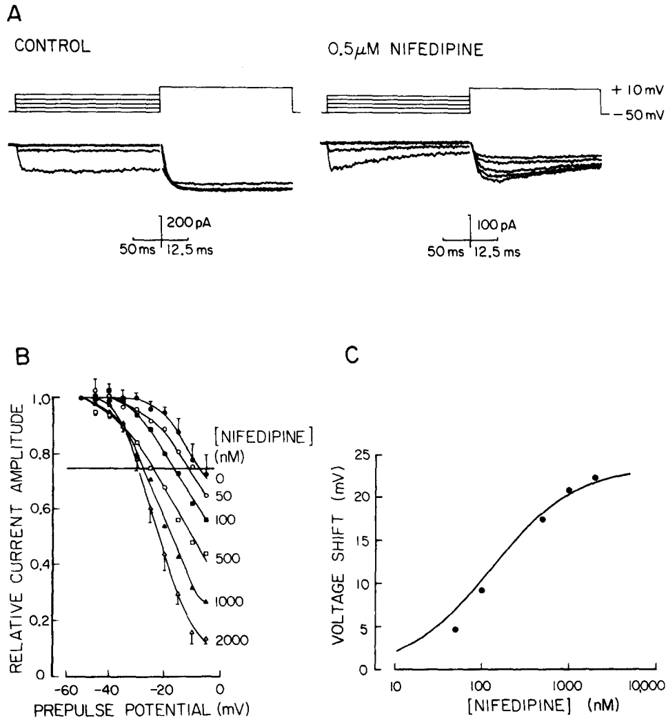
FIGURE 10. Effect of a long prepulse on \text{Ba}^{2+} current amplitude. The experimental protocol is illustrated in A . From a holding potential of -50 mV, 250-ms prepulses to various potentials were applied before depolarization to the test potential of +10 mV. In the absence of nifedipine, little inactivation of the \text{Ba}^{2+} current was observed during prepulses to -45 to -20 mV, as evidenced by the superposition of the currents elicited by the test depolarization. In the presence of 0.5 \mu\text{M} nifedipine, however, a prepulse to -30 mV was sufficient to cause substantial inactivation. In B , the peak amplitudes of I_{\text{si}} , elicited from various prepulse potentials, have been normalized to the amplitude measured when I_{\text{si}} was evoked directly from -50 mV, and are plotted as a function of prepulse potential. Results obtained in the presence of various nifedipine concentrations are shown; the horizontal line is drawn at 25% inactivation. The voltage shift of the curves in B , at 25% inactivation, is plotted as a function of nifedipine concentration in C . The solid curve represents the best fit of Eq. 2 to the data and provides an estimate of K_1 = 39 nM.
