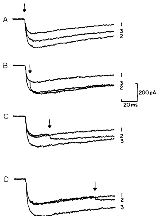
FIGURE 9. Recovery depends on the timing of the flash. In each case, three Ba^{2+} currents (labeled 1, 2, and 3), evoked 5 s apart by voltage steps from -50 to +10 mV in the presence of 0.5 \mu M nifedipine, are superimposed. In each panel, a single flash was delivered during the second trial only, at the times indicated by the arrows. When the flash was delivered before or at the peak of I_{si} (A and B), the current increased, and, in the third trial, reblocking was evident as nonirradiated nifedipine diffused to the cell. When the flash was presented after the peak current (C and D), it was less effective at removing nifedipine blockade; the third trial showed a further increase in I_{si} amplitude. In some experiments, when the flash was presented late during the voltage step, there also appeared to be a step-like component to the flash-induced current (D), a finding that suggests that a small component of the recovery may be attributed to reversal of open channel block (see Discussion).
