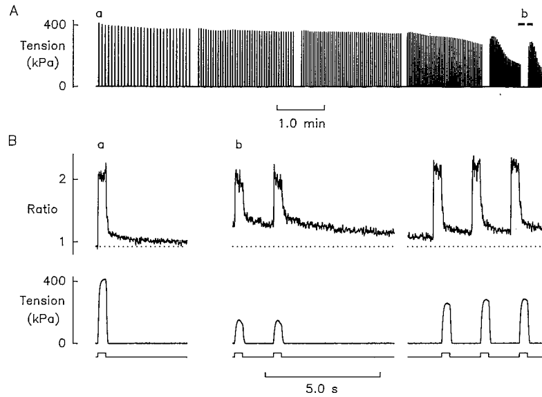
FIGURE 5. A fatigue run with 10-s rest periods. (A) Continuous tension record. (B) Records of tension and fluorescence ratio from the first tetanus ( a ) and from the last 10-s pause ( b ). Observe the marked recovery of both tension and ratio that occurred during the pause. The dotted lines represent the resting ratio in control. Stimulation periods are indicated below tension records.
