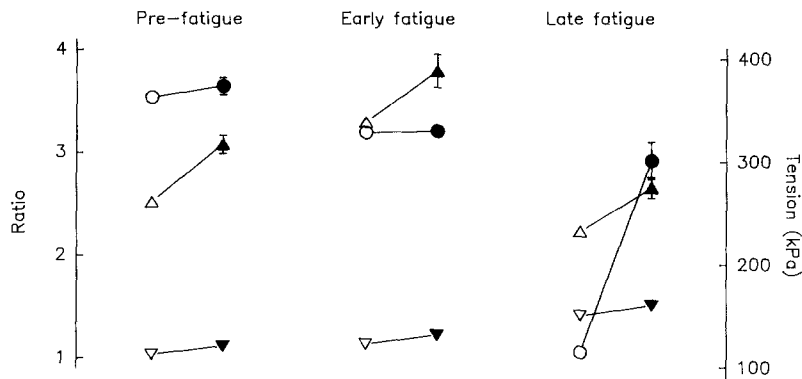
FIGURE 8. Summary of the results from caffeine application under control conditions (pre-fatigue; n = 6 ), after ~20 fatiguing tetani (early fatigue; n = 3 ), and in the fatigued state (late fatigue; n = 4 ). ○, ●, Tension; ▽, ▾, resting fluorescence ratio; △, ▲, tetanic fluorescence ratio; open and filled symbols represent values obtained before and during caffeine exposure, respectively. Values are given as mean \pm SE of the mean difference between measurements before and during caffeine exposure.
