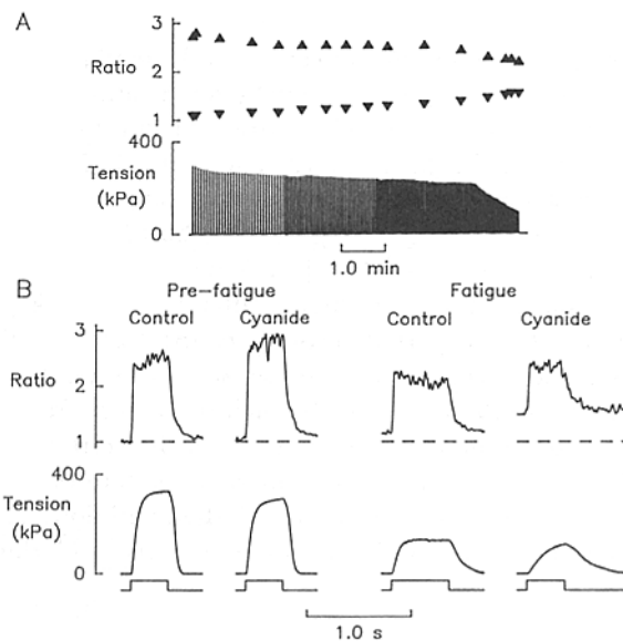
FIGURE 12. Tension and fluorescence ratio signals obtained from a fiber exposed to 2 mM cyanide. (A) A plot of resting and tetanic ratios during fatiguing stimulation and the original tension record. Observe that there was no significant early increase of the peak ratio. (B) Records selected to illustrate that exposure of rested fibers (prefatigue) to cyanide caused a small tension reduction accompanied by an increased tetanic ratio, and the resting ratio in the fatigued state was substantially higher when the fiber had been fatigued in the presence of cyanide.
