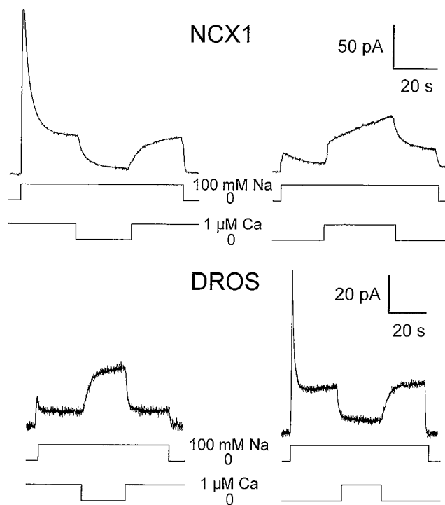
FIGURE 3. Effects of cytoplasmic \text{Ca}^{2+} on outward \text{Na}^+-\text{Ca}^{2+} exchange currents for the canine cardiac (NCX1) and Drosophila (DROS) \text{Na}^+-\text{Ca}^{2+} exchangers. All outward currents were activated by replacing 100 mM cytoplasmic \text{Cs}^+ with \text{Na}^+ ; transported \text{Ca}^{2+} (pipette) remained constant at 8 mM. Regulatory cytoplasmic \text{Ca}^{2+} (1 \mu\text{M} ) was added or removed as indicated under the current traces.
