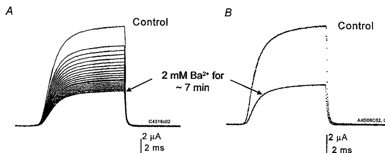
FIGURE 1. External Ba 2+ can block the closed state of ShH4-IR. (A) A depolarizing command to 30 mV was given under control conditions ( upper trace ) and at 5-s intervals after the addition of 2 mM Ba 2+ to the external solution; every fourth trace is shown. The total time of the experiment was ~7 min. (B) The upper trace was recorded under control conditions, and the lower was recorded approximately 7 min after the addition of 2 mM Ba 2+ to the external solution. In this case, Ba 2+ was added to the external solution while holding the membrane at -90 mV; this holding potential was maintained for the entire duration between the two pulses shown.
