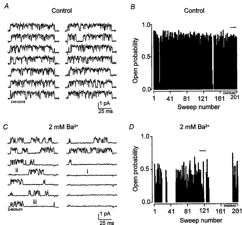
FIGURE 8. Ba 2+ introduces discrete blocked times in single-channel records. ( A and C ) Consecutive sweeps recorded in control conditions ( A ) and with 2.0 mM Ba 2+ in the pipette ( C ). The membrane was held at -90 mV and stepped to 30 mV for 100 ms, repeated once every 1 s; data are filtered at 1 kHz. In C , the lowercase roman numerals indicate three subtypes of discrete blocking events: (i) no openings, (ii) blocked times that precede channel opening, and (iii) blocked times that follow channel opening. ( B and D ) Plots of open probability versus sweep number for 200 consecutive sweeps in control conditions ( B ) and with 2.0 mM Ba 2+ in the pipette ( D ). The horizontal bars in B and D indicate the sweeps shown in A and C , respectively.
