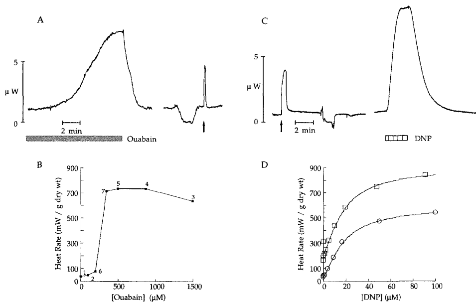
FIGURE 5. Effect of ouabain or DNP on isosmotic heat rates. (A) Original record of rate of heat production of a trabecula of dry weight 9.7 \mu\text{g} , diameter 130 \mu\text{m} and length 2.1 \text{ mm} . Resting heat rate in response to 875 \mu\text{mol liter}^{-1} ouabain (shaded rectangle); following the discontinuity: determination of basal and active (in response to 10-Hz electrical stimulation) heat rates in absence of ouabain (stimulus heat 370 \text{ nW} ). (B) heat rate as a function of ouabain concentration for same trabecula as shown in A; order of presentation of ouabain doses indicated. (C) Original record of rate of heat production of a papillary muscle of length 3.1 \text{ mm} and dry weight 15.9 \mu\text{g} . Arrow: 30 s of electrical stimulation (stimulus heat 130 \text{ nW} ); resting heat rate 0.6 \mu\text{W} ; following the discontinuity: response to
