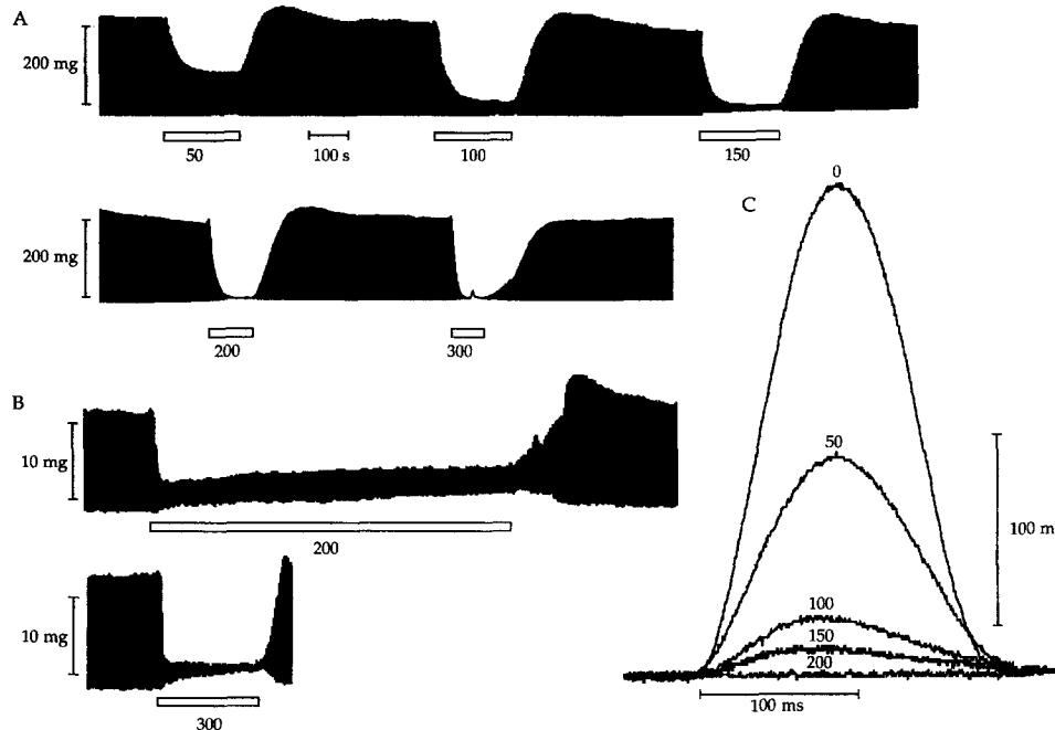
FIGURE 6. Effect of osmolality on force production. (A) Right ventricular papillary muscle of circular cross-section ( 200 \mu\text{m} diameter and 2.72 \text{ mm} length) and dry weight 24.6 \mu\text{g} . (B) Right ventricular trabecula of circular cross-section ( 100 \mu\text{m} diameter and 2.44 \text{ mm} length) and dry weight 3.1 \mu\text{g} . Preparations stimulated electrically at 2.5 \text{ Hz} ; slow chart speed fails to distinguish separate twitches. Bathing solution rendered hyperosmotic by addition of sucrose ( \text{mmol l}^{-1} ) for periods indicated by open rectangles. (C) Selected steady-state twitches, recorded at higher speed and gain, from A.
