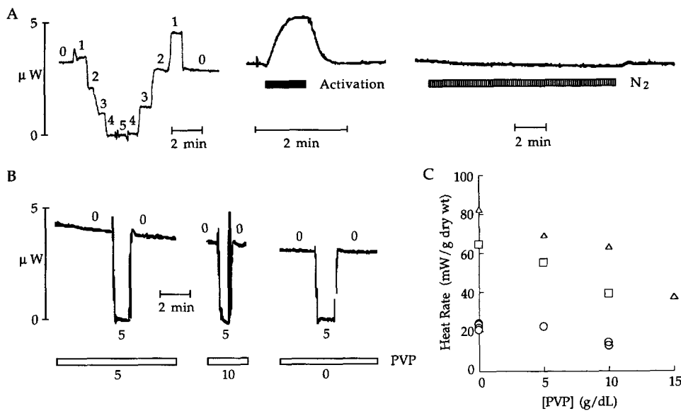
FIGURE 8. Effect of osmolality on rate of heat production of chemically skinned trabeculae. (A) Original record from a cylindrical trabecula (diameter 250 \mu\text{m} , length 2.0 mm and dry weight 128.8 \mu\text{g} ) that had been immersed in skinning solution for 80 min) superfused with relaxing solution and moved (in steps of 1 mm, as indicated) 5 mm downstream out of the measurement chamber and returned; resting heat rate 3 \text{mW g}^{-1} . After the first discontinuity: preparation exposed to activating solution for 1 min then to 100% \text{N}_2 in relaxing solution for 10 min. (B) Same trabecula as in A, bathed in relaxing solution containing PVP in concentrations ( \text{g dl}^{-1} ) indicated, moved in single steps of 5 mm down-
