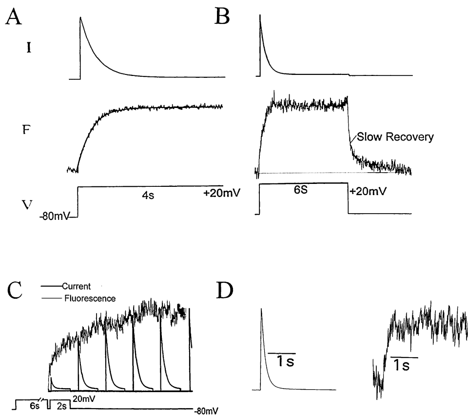
FIGURE 1. Correlation of slow inactivation of ionic current and fluorescence of 424C-TMRM channels. (A) Fluorescence ( F ) increases during a voltage step ( V ) with the kinetics of current ( I ) inactivation (solid line superimposed on fluorescence trace is time course of current inactivation from a monoexponential fit). Tau for the fluorescence was 300 \pm 22 ( n = 7 ) and the Tau for the current decay was 289 \pm 31 ( n = 6 ). (B) Upon repolarization, fluorescence recovery consists of fast and slow components. (C) The slow component of fluorescence recovery follows the kinetics of recovery of the ionic current. The slow component of fluorescence recovery ( noisy trace ) was taken from B , starting at point indicated, and inverted and superimposed on a series of currents evoked by identical test depolarizations ( bottom ) given at varying intervals after a 6-s depolarization (not shown). The Taus for the current recovery and fluorescence decay were 2,344 \pm 212 and 2,363 \pm 205 ms ( n = 3 ), respectively. (D) Fluorescence follows current inactivation in chan-
