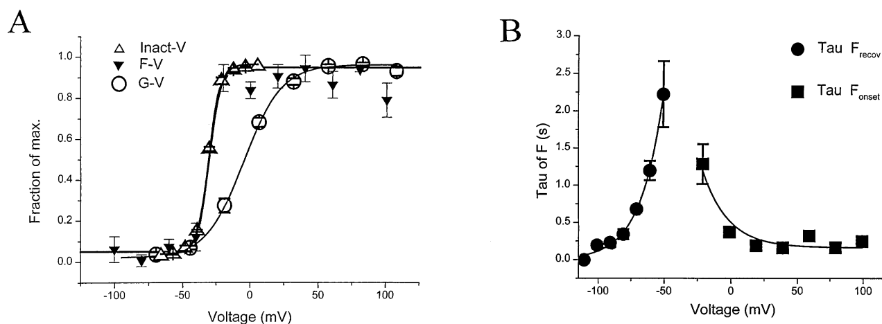
FIGURE 3. Voltage dependence of current inactivation and 424C-TMRM fluorescence. (A) Voltage dependencies of channel opening (G-V), fluorescence (F-V), and current inactivation (Inact-V). The F-V relations were obtained from measurements of fluorescence 4 s after the start of a step to the indicated test potential (long enough for the fluorescence change to reach steady state at all test potentials). Inact-V relations were obtained from a measure of the fraction of the maximal decline in current evoked by a step to +20 mV, following a 4-s prepulse to the indicated test potential. The G-V was calculated from steady state, leak-subtracted currents assuming E_k = -100 mV. Measurements made in W434/424C-TMRM channels ( n = 10 ). Fits are to single Boltzmann functions. (B) Voltage dependence of the time constants for F_{\text{onset}} (measured from 4-s depolarizations) and F_{\text{reco}} (measured from 20-s long tails to indicated potentials, after a 4-s depolarization to 0 mV). Rate of F_{\text{onset}} appears to be intrinsically voltage independent since it does not change over a wide range of positive potentials. Fits are to single exponentials.
