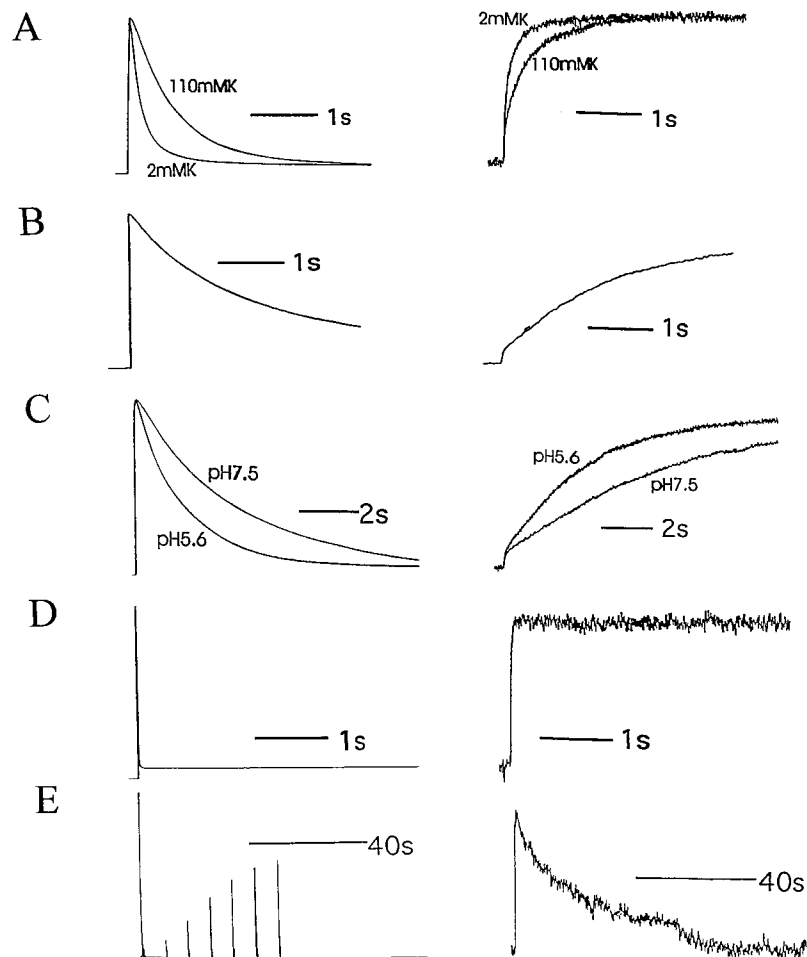
FIGURE 2. 424C-TMRM fluorescence (right) follows ionic current inactivation (left) under molecular and ionic conditions that alter inactivation rate. (A) Exchange of external solution from 2 to 110 mM K + slowed both current inactivation and the rate of fluorescence increase of 424C-TMRM/W434/C462A channels ( \tau_{\text{ion-onset (110K)}} = 742 \pm 54 ms, n = 6 ); \tau_{\text{fluor-onset (110K)}} = 689 \pm 28 ms, n = 6 . (B) Channels with a cysteine restored at position 462 (424C-TMRM/W434/C462) were equally slow in current inactivation and fluorescence increase ( \tau_{\text{ion-onset (C462)}} = 2,476 \pm 345 ms; \tau_{\text{fluor-onset (C462)}} = 2,412 \pm 407 ms, n = 10 ). (C) Exchange of external solution from pH 7.5 to 5.6 accelerated both current inactivation and the rate of fluorescence increase of 424C-TMRM/W434/C462 channels. (D and E) Restoration of the NH 2 -terminal fast inactivation ball to 424C-TMRM/W434/C462A channels accelerated current inactivation and the rate of fluorescence increase (D) and slowed current and fluorescence recovery (E) compared with control (see Fig. 1). ( \tau_{\text{ion-onset (+ball)}} = 14 \pm 2 ms; \tau_{\text{fluor-onset (+ball)}} = 45 \pm 3 ms; n = 8 .)
