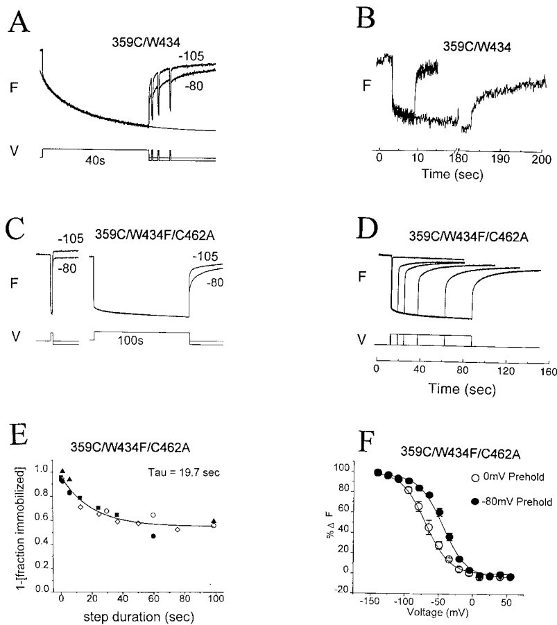
(E) Relation of reduction in amplitude (immobilization) of the fast component of F_{\text{recovery}} to step duration, measured from traces such as D . Data from five oocytes (each oocyte = one symbol) combined and fit to a single exponential (solid line). (F) Long (2-min) predepolarization (to 0 mV) shifts, in the negative direction, the voltage dependence of the fast fluorescence-voltage relation. Fluorescence was measured at the end of 200-ms steps to indicated potentials that are primarily from the fast component of fluorescence change. Steps were given at 4-s intervals to permit recovery from small amounts of inactivation induced by positive steps from V_{\text{hold}} = -80 mV, or to permit re-entry into the inactivated state after small amounts of recovery during negative steps from V_{\text{hold}} = 0 mV. Data from five oocytes. Note that return to a more negative ( -105 mV) tail potential than V_{\text{hold}} ( -80 mV) makes the fast component larger in the recovery for both W434 (A) and W434F/C462A (C) because a larger fraction of S4s enter their resting conformation.
