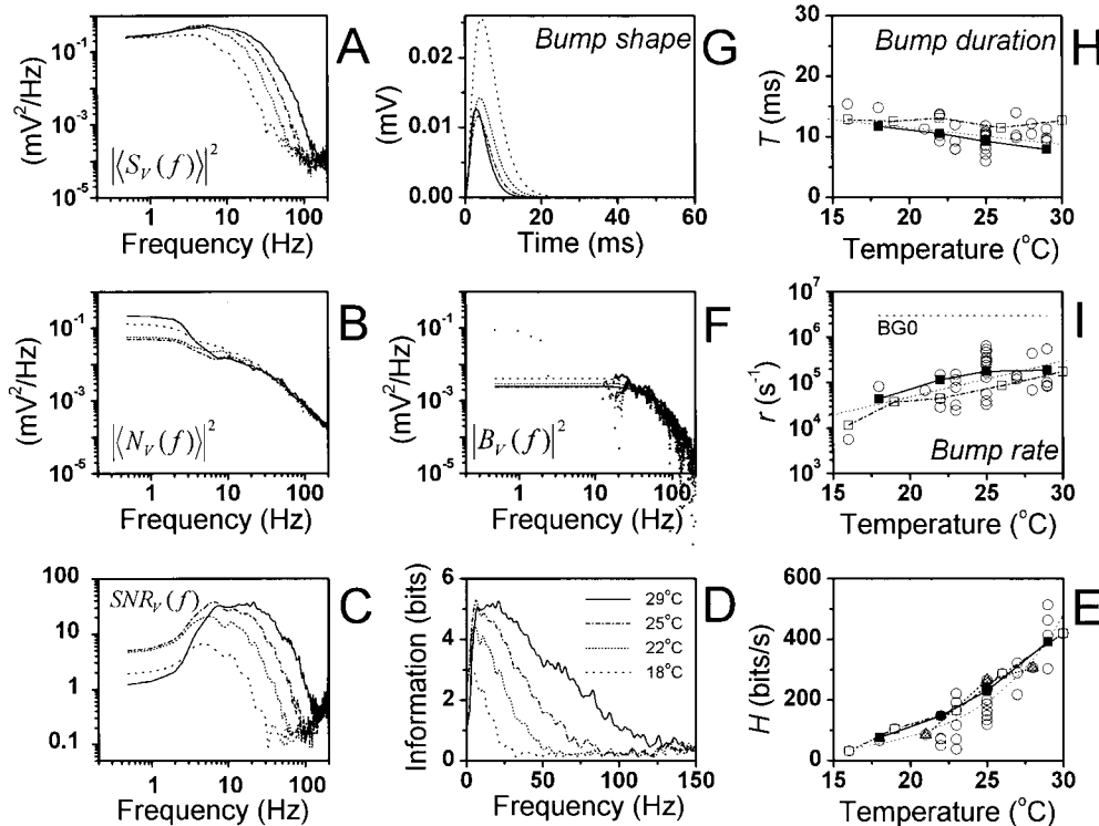
FIGURE 4. The photoreceptor response dynamics at BG0 at different temperatures. (A) The signal power spectra, |\langle S_V(f) \rangle|^2 , (B) noise power spectra, |\langle N_V(f) \rangle|^2 , and (C) SNR_V(f) calculated via the FFT (see Juusola and Hardie, 2001). (D) The information at different temperatures, \log_2[SNR_V(f) + 1] , and (E) the information capacity, the integral of the information over all frequencies (Juusola and Hardie, 2001). (F) The bump noise power (continuous lines) was isolated by subtracting the photoreceptor noise power spectrum, measured at darkness, from the power spectrum, measured at the BG0, and fitted with single Lorentzians (dotted lines). This gives us the two parameters ( n and \tau ) for calculating the bump shape (G) and the effective bump duration (H) at BG0 (the symbols indicate the photoreceptors as previously described). The bump event rate (I) was estimated as described in the text (Eq. 6).
